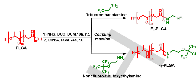
Scheme 1. Synthesis and chemical structures of the fluorinated PLGA (F-PLGA) derivatives: \text{F}_3 -PLGA and \text{F}_9 -PLGA.
