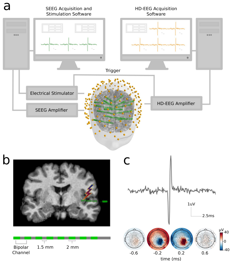
Fig. 1 Illustration of the experimental setup. (a) Depiction of the stimulation and acquisition systems' temporal synchronization and spatial co-registration. (b) Top: example of an intracerebral shaft containing eight contacts coregistered with the subject's MRI. Bottom: Illustration of an intracranial shaft. (c) Top: Example of a stimulation artifact recorded by a scalp EEG channel. Bottom: Scalp EEG topographies at the time of the stimulation onset.
