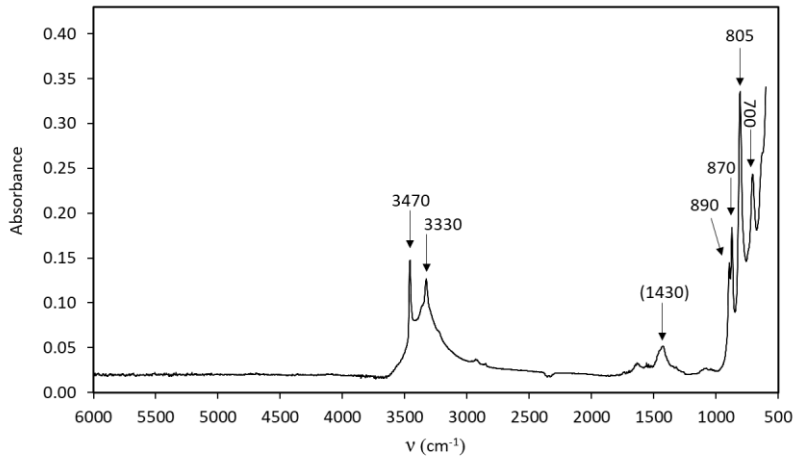
Fig. 2. FTIR spectrum (powder sample with KBr) of langhofite. The broad band at ca. 1430 \text{cm}^{-1} is relate to a carbonate impurity.
