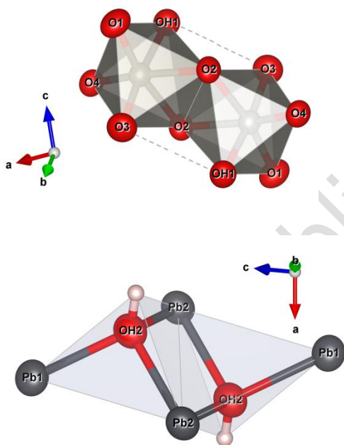
Fig. 6. Polyhedral representation of the [W_2O_8(OH)_2]^{6-} (a) and [(OH)_2Pb_4]^{6+} (b) dimers. Diagram obtained with Vesta 3.0 (Momma and Izumi, 2011).
