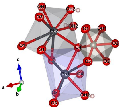
Fig. 5. The coordination environment of the two Pb sites and the W site in the structure of langhofite. The stronger (shorter) bonds are shown in red. Diagram obtained with Vesta 3.0 (Momma and Izumi, 2011).
