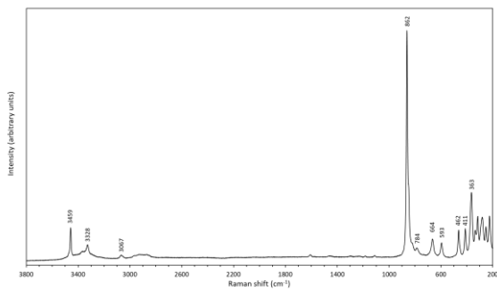
Fig. 4. Raman spectrum of langhofite, random section.
