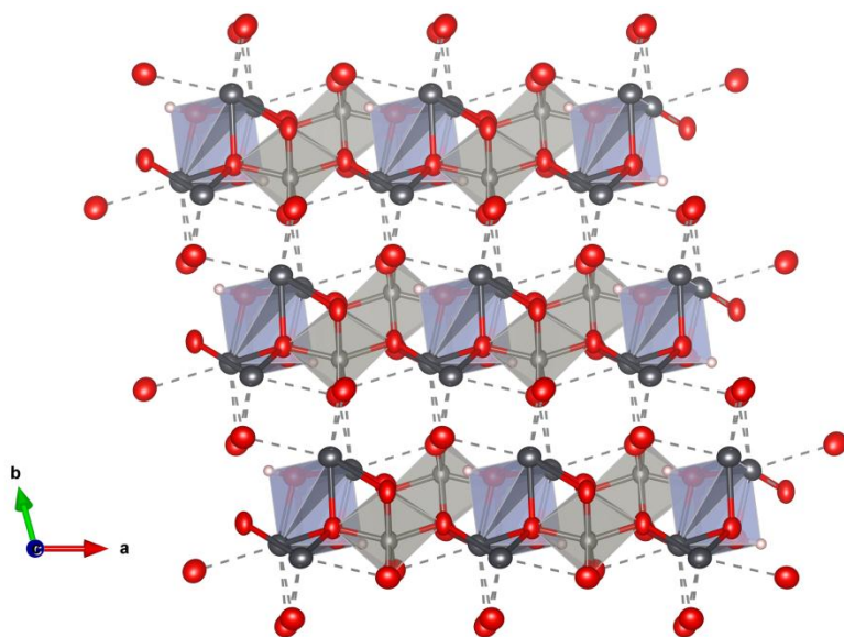
Fig. 8. The layered structure of langhofite: the (010) layers are linked along [010] through the weaker longer Pb-O bonds (shown with dashed lines). Diagram obtained with Vesta 3.0 (Momma and Izumi, 2011).
