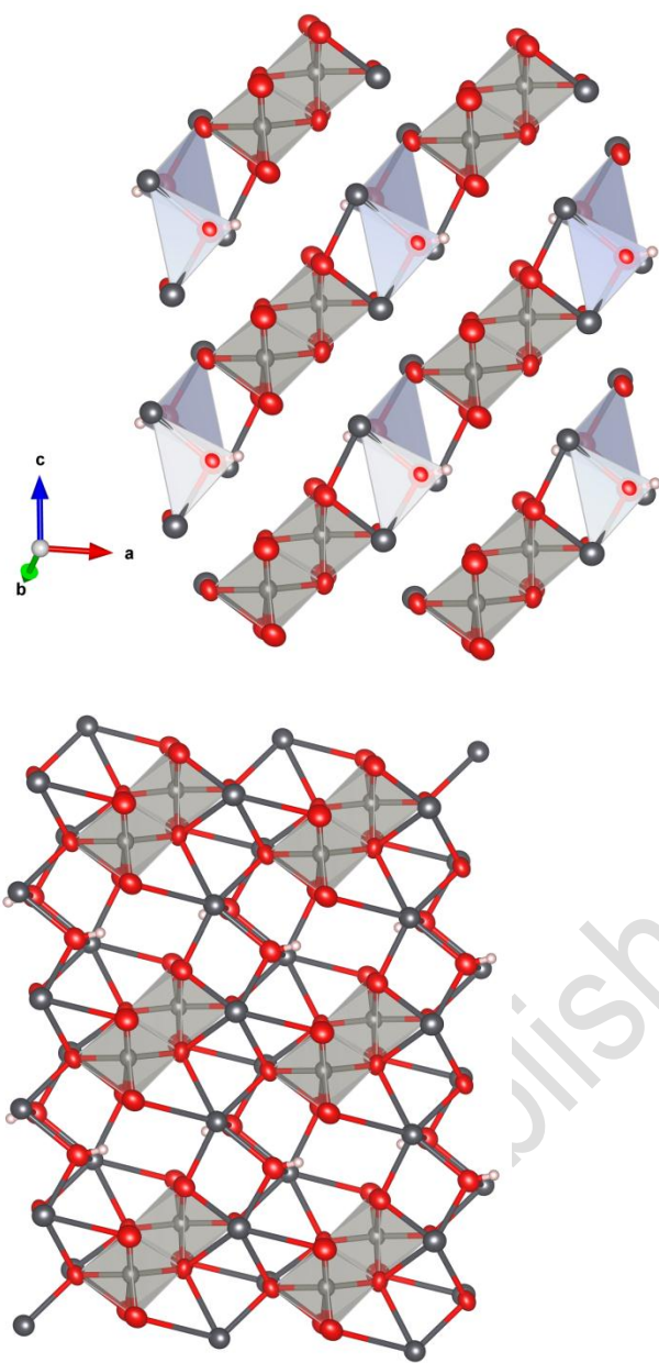
Fig. 7. The [\text{W}_2\text{O}_8(\text{OH})_2]^{6-} and [(\text{OH})_2\text{Pb}_4]^{6+} units forming chains along [101] in langhofite (a). The chains configure (010) layers when all the strong Pb-O bonds are considered (b). Diagram obtained with Vesta 3.0 (Momma and Izumi, 2011).
