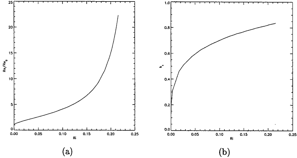
Figure 2: Critical Reynolds number (a) and critical wave number (b) as functions of Richardson number for \text{Pr} = 10 for the periodic case.
