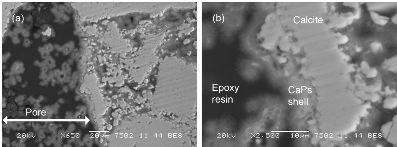
Fig.1 SEM images (BS) collected on polished cross section of Noto limestone treated with the DAP solution and showing the nucleation of the shell of calcium phosphates in a pore within the matrix (a) and detail at higher magnification (b). The SEM images are collected at a depth of 3 mm.
