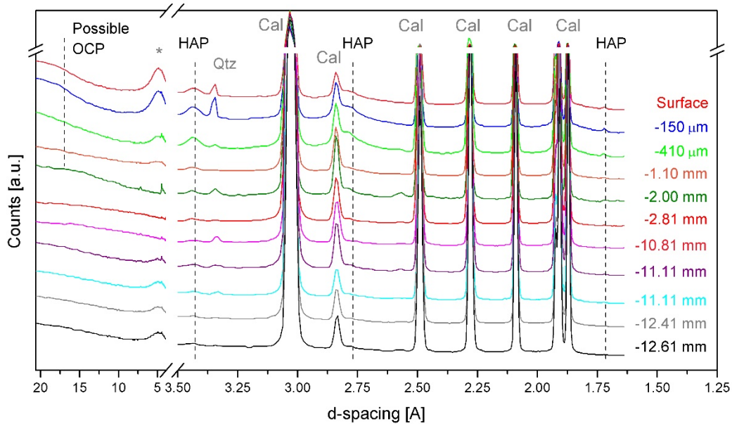
Fig. 3 SR- \mu TXRD patterns of treated Noto limestone from the surface down to 12.61 mm depth, showing the unambiguous presence HAP peaks. Possible peaks due to OCP are showed as well. Cal = calcite, Qtz = quartz, * = clay minerals.
