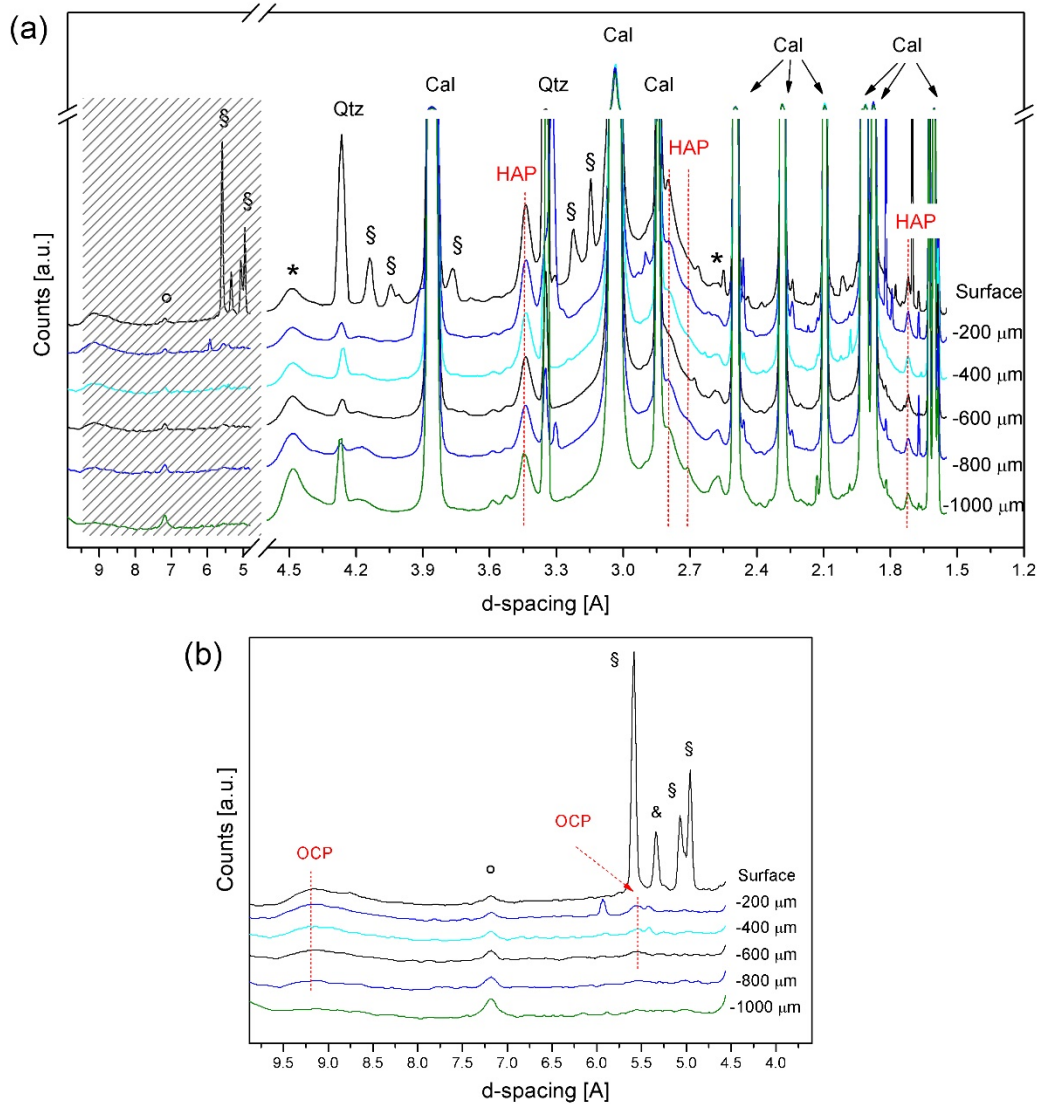
Fig. 4 SR- \mu TXRD patterns at different depth from the surface of treated Noto limestone (a). Zoom of the SR- \mu TXRD patterns in the region at high interplanar distances (b). Cal = calcite, Qtz = quartz, HAP = hydroxyapatite, OCP = octacalcium phosphate, * = clay minerals (smectite/montmorillonite or illite), ° = kaolinite, § = unreacted DAP, & = unreacted ADP. HAP is present in all the patterns, while OCP is present from the surface down to 600-800 micrometers.
