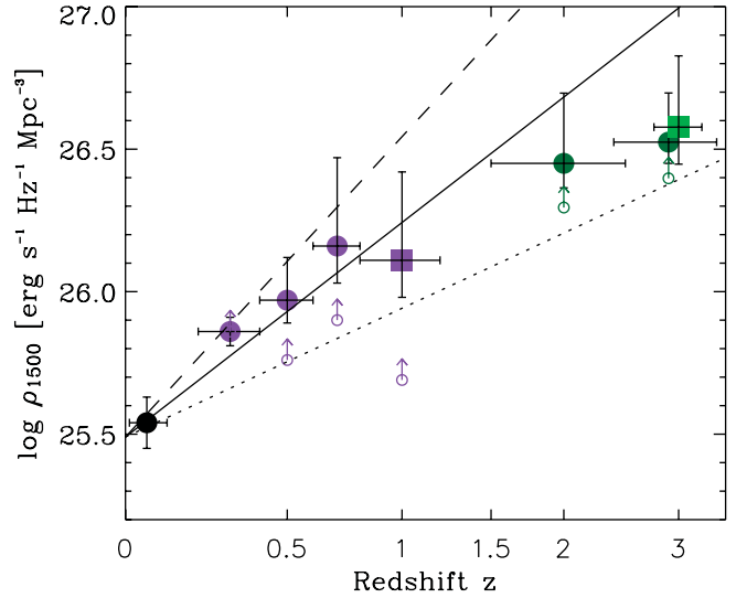
FIG. 1.—FUV LD vs. redshift. Filled circles indicate LF fit to full sample with unconstrained slope \alpha . Filled squares denote LF fit with fixed \alpha = -1.6 . Purple ( GALEX ) and dark green (HDF) symbols are from this work. Black filled circle (bottom left) is taken from local LF (Wyder et al. 2005) and green square from Steidel et al. (1999). Open circles denote \rho_{1500} determined using V_{\max} . Errors do not include cosmic variance. Lines indicate (1+z)^n evolution. Dotted, solid, and dashed lines correspond to n = 1.5, 2.5, and 3.5 , respectively.
