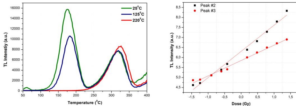
Figure 1: (Left): BeO TLD dose response curves which were obtained in three different irradiation temperatures (25 o C, 125 o C, 220 o C) for a dose of 0.38 Gy.
