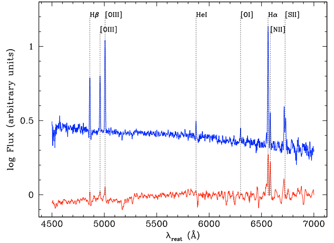
Fig. 17. Stacked spectra for galaxies with MRS elliptical morphology ( \mathcal{MT} = 1 ) and blue colours ( \mathcal{PT} = 2 + 3 + 4 ) at low-mass ( \log(M/M_{\odot}) < 9 upper spectrum in blue) and high-mass ( \log(M/M_{\odot}) > 10.5 lower spectrum in red).
