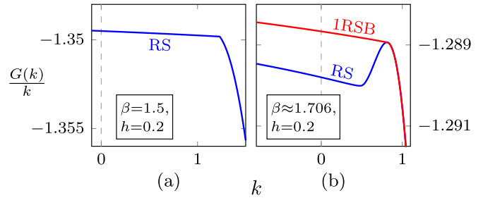
FIG. 3. The function G(k)/k for the ( p=3 )-spin in a magnetic field h=0.2 , for different values of \beta : (a) \beta=1.5 < \beta_c(h) , (b) \beta \approx 1.706, \beta_c(h=0) > \beta_c(h) . The application of a magnetic field washes out the linear behavior at small k observed in zero magnetic field.
