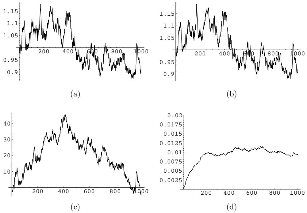
Figure 1: For \alpha = \beta = 1 , \gamma = 0.01 , x_0 = \alpha/\beta (the equilibrium solution for zero noise) and a specific realization of w(t) we show: (a) the direct numerical solution x(t) ; (b) the solution \hat{x}(t) obtained by our procedure; (c) the realization of the driving stochastic process w(t) ; (d) the relative error |\hat{x}(t) - x(t)|/x(t) . The numerical integrations are performed over 1.000 steps.
