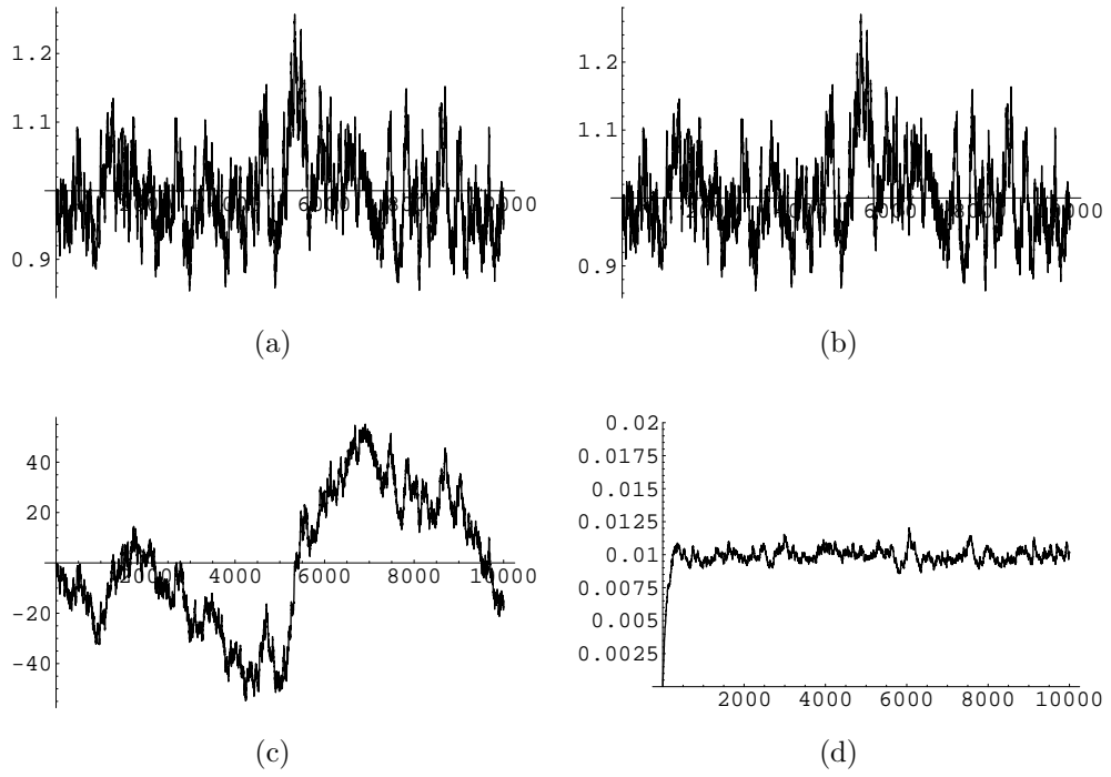
Figure 2: For the same parameters values as in Fig.1 we show again: (a) x(t) ; (b) \hat{x}(t) ; (c) w(t) ; (d) |\hat{x}(t) - x(t)|/x(t) . Here the numerical integrations are performed over 10.000 steps.
