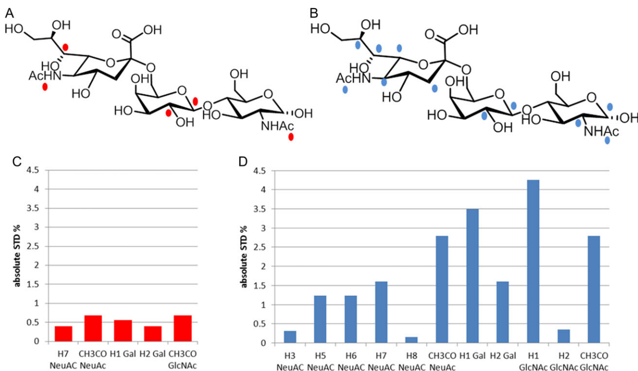
Fig. 4. The protons belonging to the epitope of compound 1 in the presence of H1-293 T cells are marked with dots (A) and the absolute STD percentage for each protons is reported (C). The same compound analyzed in presence of H5-293 T shows a stronger affinity: the epitope comprises several protons (B) with a higher intensity of absolute STD % (D).
