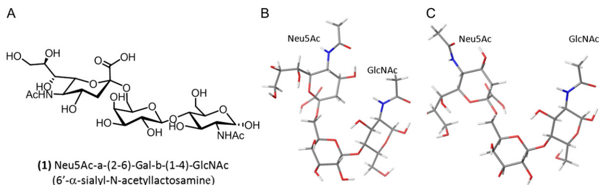
Fig. 1. Structure of Neu5Ac- \alpha -(2,6)-Gal- \beta -(1-4)-GlcNAc 1 (A). Representative structure of the bent conformation in which the distance between NeuAc H5/ GlcNAc COCH 3 is lower than 0.5 nm, compatible with the presence of the NOE (the population of this family of structure is estimated around 15%) (B). Representative structure of a more extended conformation (C).
