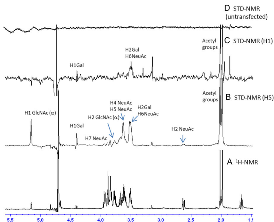
Fig. 3. (A) ^1\text{H-NMR} of 6'- \alpha -sialyl- N -acetylglucosamine in deuterated phosphate buffer pH = 7.4 ( T = 298\text{ K} ). (B and C) STD-NMR experiments of 6'- \alpha -sialyl- N -acetylglucosamine in presence of H5-293 T and H1-293 T cells respectively. (D) STD-NMR experiments of 6'- \alpha -sialyl- N -acetylglucosamine in the presence of untransfected cells. NMR experiments were performed using a Bruker 600 MHz spectrometer, STD spectra were obtained with -0.05\text{ ppm} as irradiation frequency and 2.94 s of saturation time.
