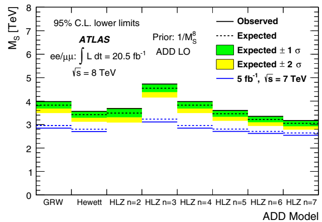
Fig. 5 Summary of 95 % C.L. lower exclusion limits on M_S for the combined dilepton ADD large extra dimensions search, using a uniform positive prior in 1/M_S^8 . Previous ATLAS search results [17] are also presented for comparison. Exclusion limits were not previously set on the HLZ n = 2 ADD model
