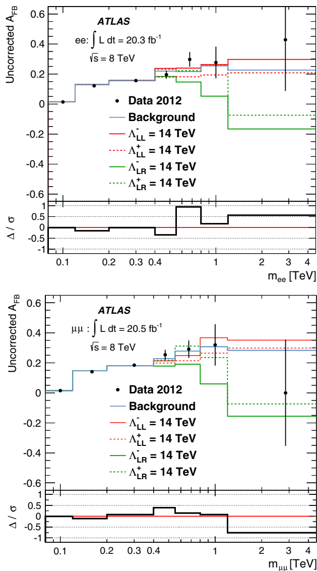
Fig. 3 Reconstructed A_{FB} distributions for data and the SM background estimate as a function of dielectron ( top ) and dimuon ( bottom ) mass. Also shown are the predictions of different benchmark \Lambda values for the LL and LR contact interaction model (the RR model is very similar to the LL case). The ratio displays the background-subtracted data ( \Delta ) divided by the total uncertainty ( \sigma ) in each bin
