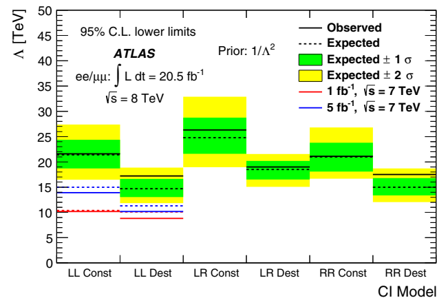
Fig. 4 Summary of 95 % C.L. lower exclusion limits on \Lambda for the combined dilepton contact interaction search, using a uniform positive prior in 1/\Lambda^2 . Previous ATLAS search results [17, 49] are also presented for comparison. Exclusion limits were previously only set on the LL model
