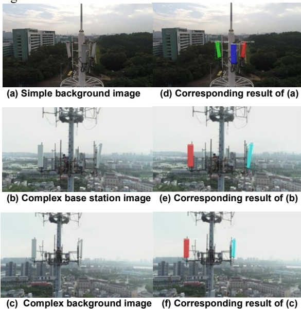
FIGURE 2. (a)-(c) are Original Antenna Images and (d)-(f) are Segmented Antenna Images
