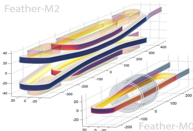
Fig. 1. Aligned block development HTS magnets, (bottom right) Feather-M0 quench detection development coil, (top left) Feather-M2 the EuCARD-2 five Tesla standalone approaching accelerator field quality insert magnet.
