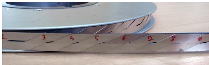
Fig. 2. Roebel cable, 20 m, dummy stainless steel, supplied by Karlsruhe Institute of Technology Institute for Technical Physics (KIT).
