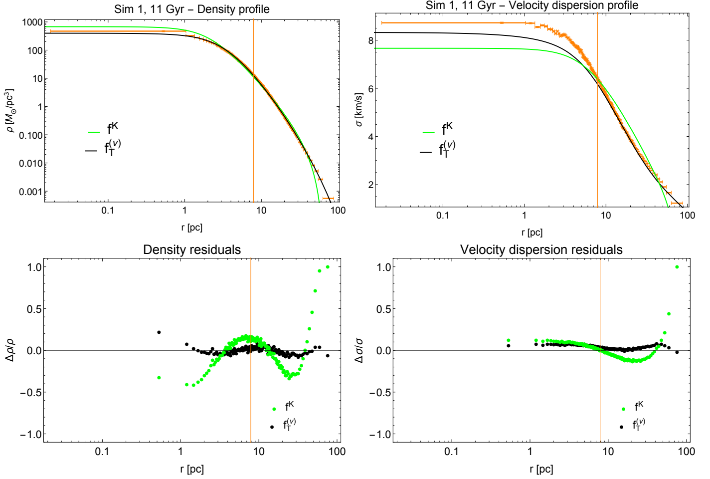
Fig. A.1. Best-fit profiles and residuals for Sim 1 at 11 Gyr for one-component King models (green) and for one-component f_T^{(v)} models (black). Upper panels: density (left) and velocity dispersion (right) profiles. Lower panels: density (left) and velocity dispersion (right) residuals.
