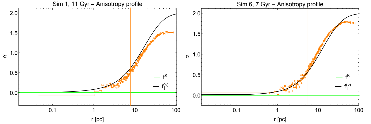
Fig. A.3. Anisotropy profiles of Sim 1 at 11 Gyr (left panel) and Sim 6 at 7 Gyr (right panel) compared to those associated with best-fit one-component f_T^{(v)} models (black) and the isotropic King models (green).
