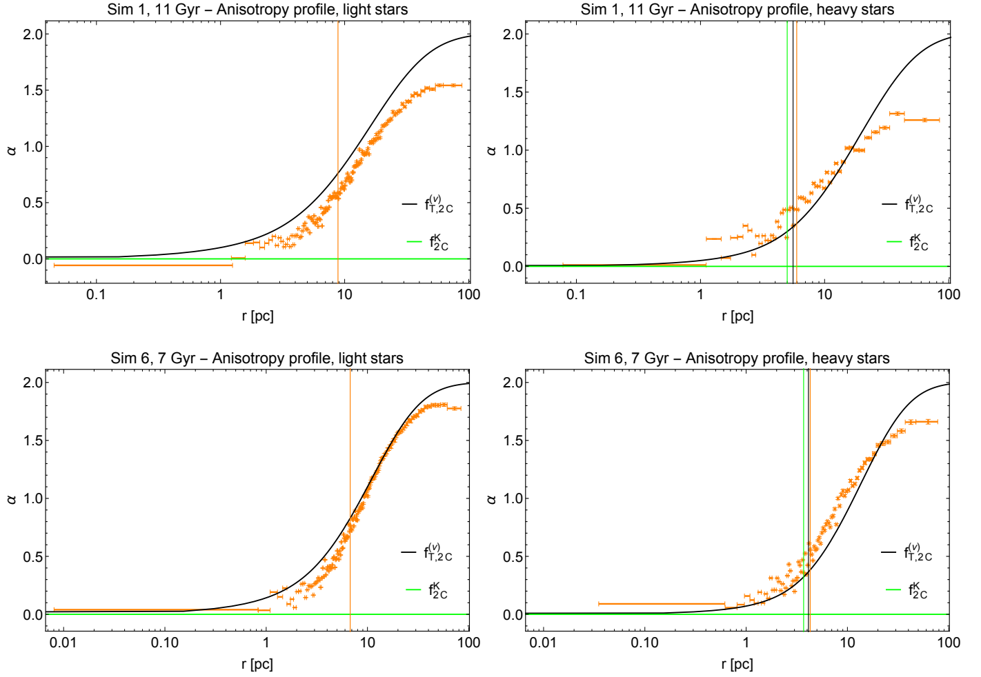
Fig. 11. Anisotropy profiles for Sim 1 at 11 Gyr (upper panels) and Sim 6 at 7 Gyr (lower panels) compared to those associated with best-fit two-component f_T^{(v)} models (black) and the isotropic King models (green). Left panels: anisotropy profiles of light components. Right panels: anisotropy profiles of heavy components. The vertical lines represent the half-mass radius of the component under consideration in the simulated states and in the models.
