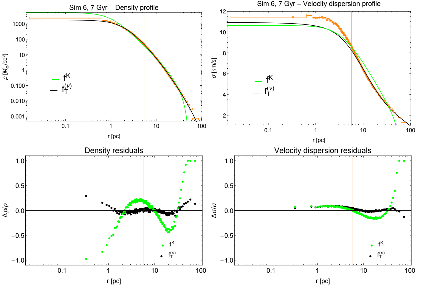
Fig. A.2. Best-fit profiles and residuals for Sim 6 at 7 Gyr for one-component King models (green) and for one-component f_T^{(v)} models (black). Upper panels: density (left) and velocity dispersion (right) profiles. Lower panels: density (left) and velocity dispersion (right) residuals.
