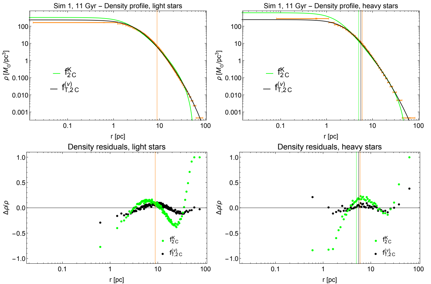
Fig. 7. Best-fit profiles and residuals for Sim 1 at 11 Gyr for two-component King models (green) and for two-component f_T^{(v)} models (black). Upper panels: density profile for light component (left) and for heavy component (right). Lower panels: density residuals for light component (left) and for heavy component (right). Vertical lines represent the half-mass radius of the component under consideration in the simulated state and in the models.
