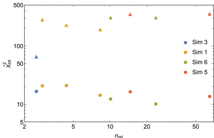
Fig. 6. Values of \bar{\chi}_{tot}^2 (plotted against n_{rel} ) associated with two-component King models (triangles) and f_T^{(v)} models (circles). The plot shows that the latter models perform far better than the former models.
