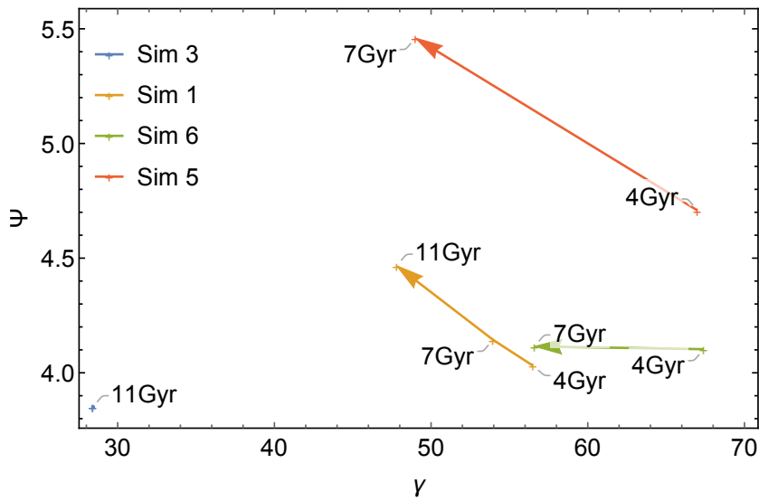
Fig. 12. Distribution of best-fit two-component f_T^{(v)} models in the relevant parameter space. The arrows connect different snapshots of the same simulation.
