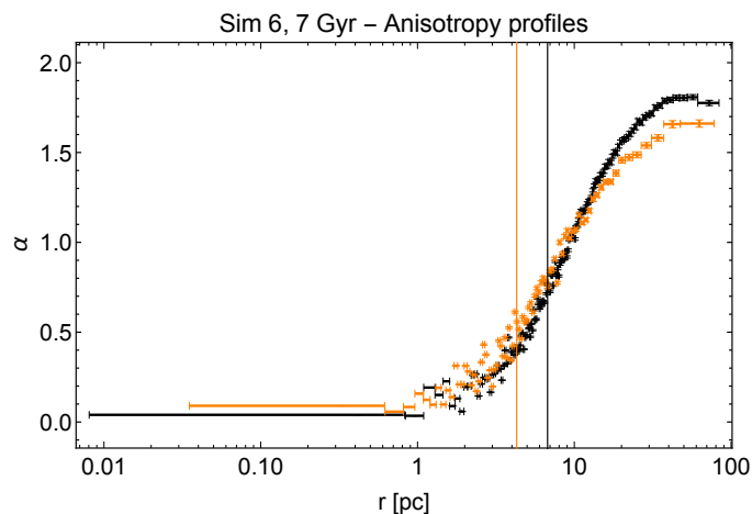
Fig. 4. Anisotropy profiles for light (black) and heavy (orange) component of Sim 6 at 7 Gyr. Uncertainties on the profile values are obtained by propagating the errors on the different velocity dispersions. The vertical lines indicate the half-mass radius of the component under consideration.
