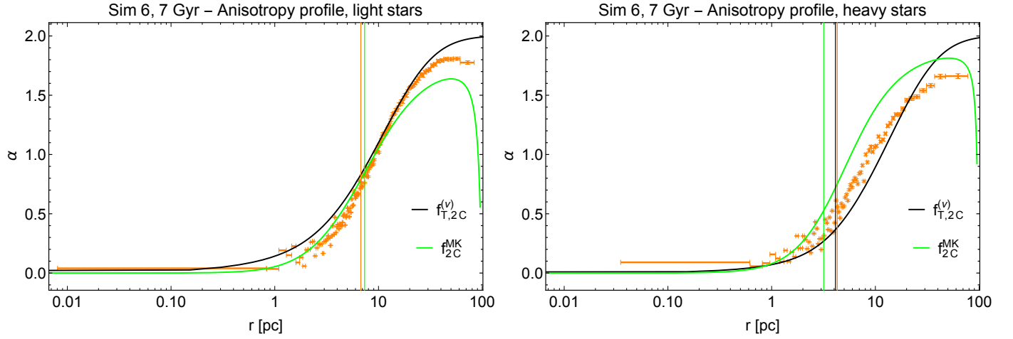
Fig. B.3. Anisotropy profiles Sim 6 at 7 Gyr compared to those associated with best-fit two-component f_T^{(v)} models (black) and Michie-King models (green). Left panel: anisotropy profile of light component. Right panel: anisotropy profiles of heavy component. The vertical lines represent the half-mass radius of the component under consideration in the simulated states and in the models.
