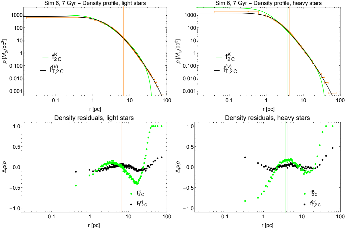
Fig. 9. Best-fit profiles and residuals for Sim 6 at 7 Gyr for two-component King models (green) and for two-component J_T^{(v)} models (black). Upper panels: density profile for light component (left) and for heavy component (right). Lower panels: density residuals for light component (left) and for heavy component (right). The vertical lines represent the half-mass radius of the component under consideration in the simulated state and in the models.
