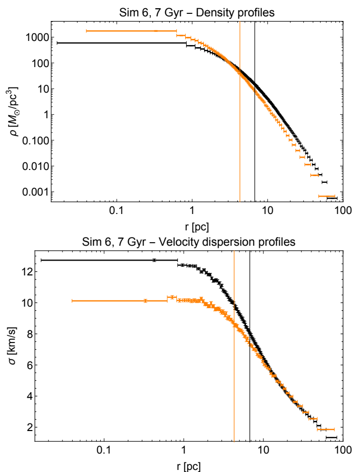
Fig. 3. Density (upper panel) and velocity dispersion (lower panel) profiles for light (black) and heavy (orange) component of Sim 6 at 7 Gyr. Uncertainties on the profile values are obtained by means of a bootstrap resampling. The differences between the two density profiles indicate the presence of mass segregation, whereas the differences between the two velocity dispersion profiles may be interpreted as due to the effects of partial energy equipartition. The vertical lines indicate the half-mass radius of the component under consideration.
