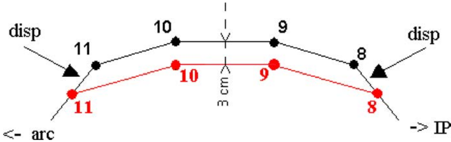
Fig. 2.15. Effect of displacing the DS dipole pairs 8 and 11, to make space for TLCD collimators, on the local footprint [46].
