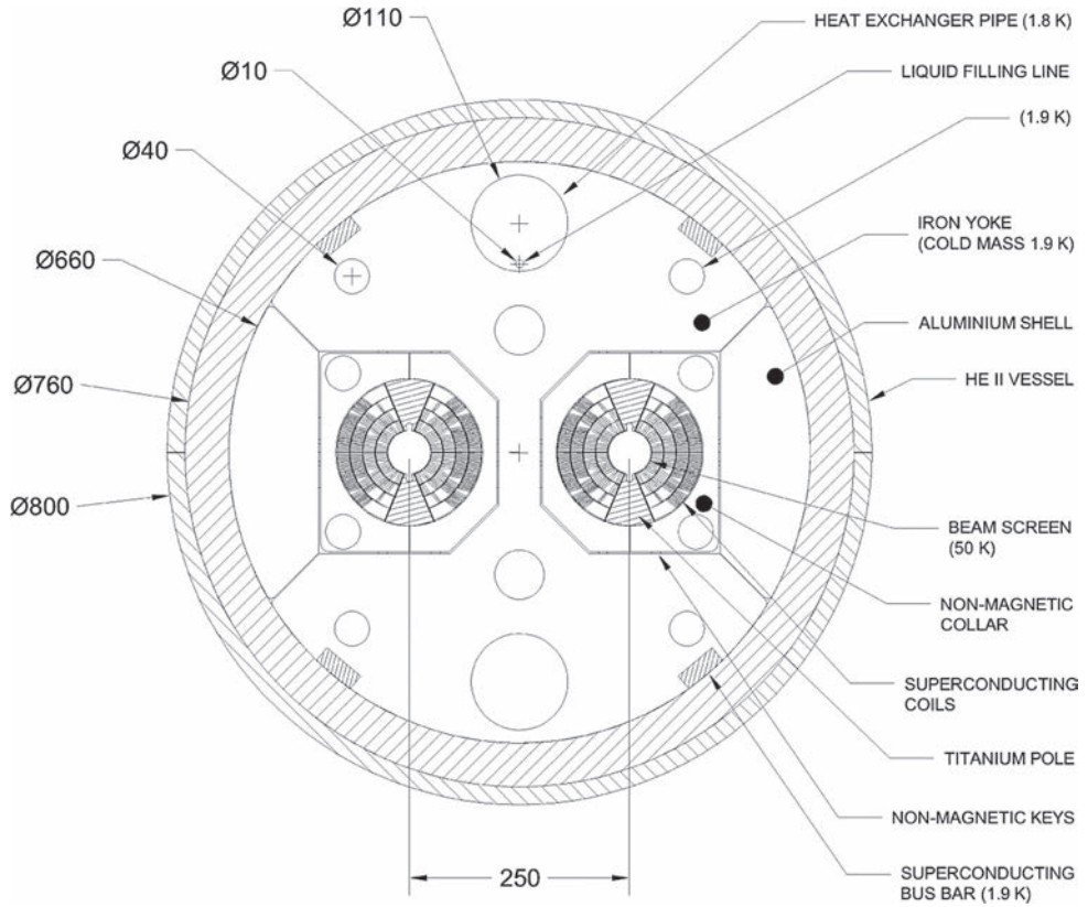
Fig. 3.4. Main dipole cold mass.
