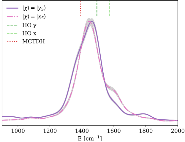
FIG. 5. Semiclassical power spectra in the shared proton perpendicular mode region, employing symmetrized reference states of type (iv) and multi-reference trajectory sampling, as explained in Sec. III D. The straight dashed lines correspond to the non degenerate harmonic frequencies of the 8th and 9th normal modes. The dotted line indicates the MCTDH result from Ref. 44. Gray bands behind the curves indicate the standard deviation of the estimated spectra.
