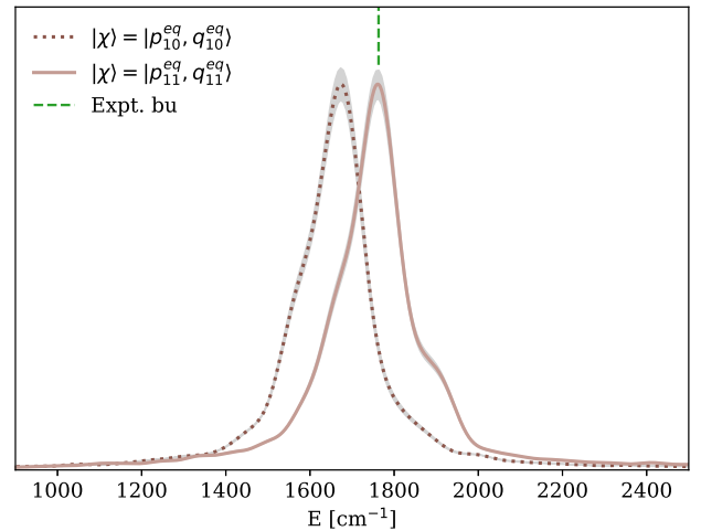
FIG. 2. Semiclassical power spectra in the bendings' region. Curves refer to different reference coherent states and trajectory sampling, as explained in Sec. III B. The straight dashed line corresponds to the experimental result of Ref. 32 for optically active bending band. Gray bands behind the curves indicate the standard deviation of the estimated spectra.
