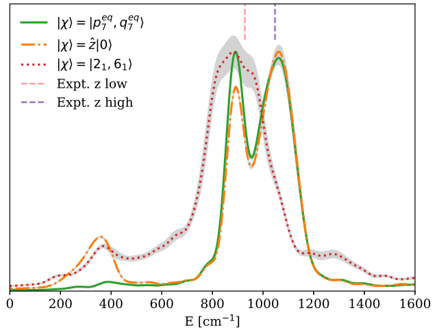
FIG. 3. Semiclassical power spectra in the proton transfer region. Curves refer to different reference states, of types (i), (iii), and (ii), respectively. The corresponding trajectory sampling is described in Sec. III C. The straight dashed lines correspond to the experimental result of Ref. 32 for the proton transfer doublet. Gray bands behind the curves indicate the standard deviation of the estimated spectra.
