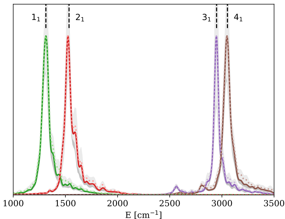
FIG. 1: Semiclassical power spectrum of the fundamental vibrational states of methane (arbitrary units on the vertical axis).
