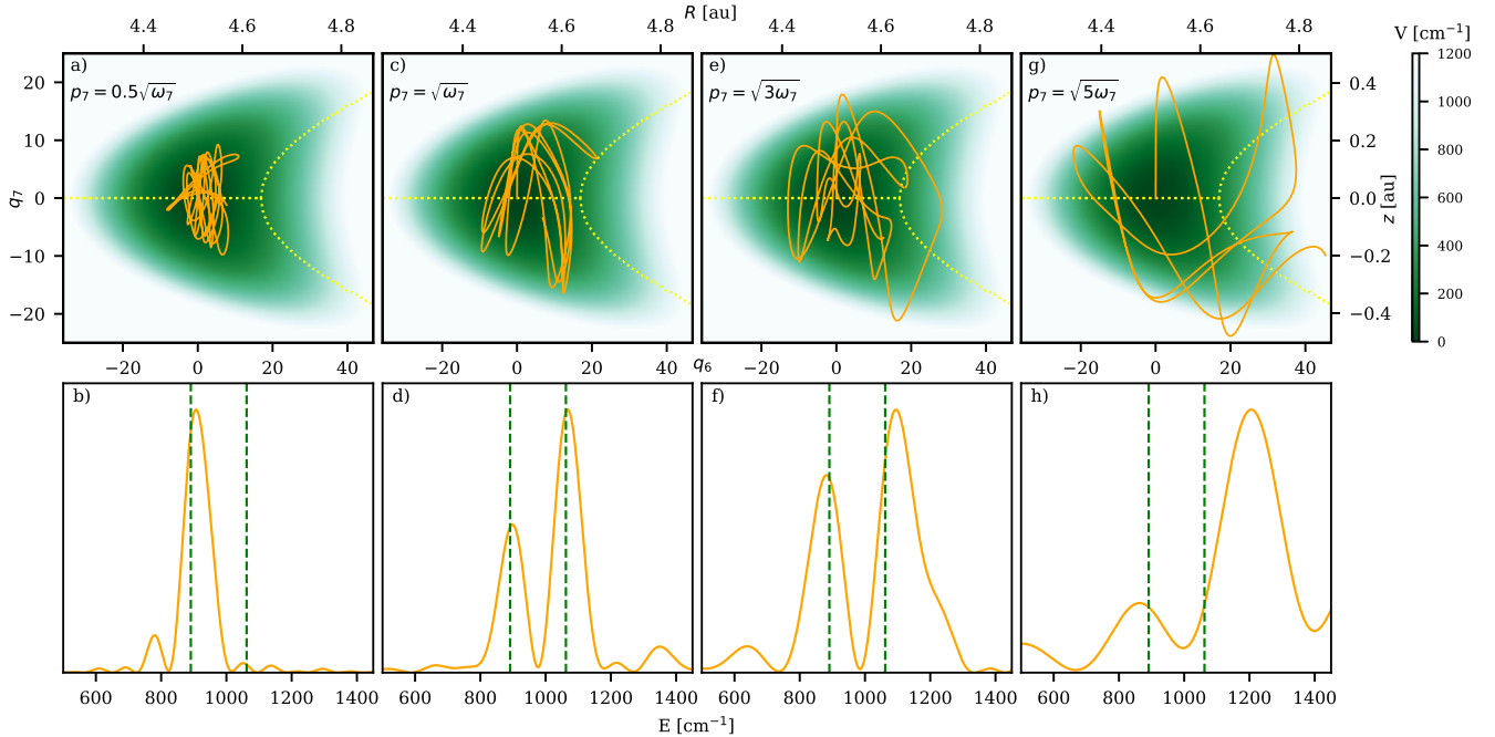
FIG. 7. Upper panels (a, c, e, g): density plot of a section of the PES with all normal modes set to equilibrium except for modes q_6 (O-O stretching) and q_7 (proton transfer); top and right axes show the corresponding R and z coordinates; for each value of q_6 , the minima of the PES with varying q_7 are indicated (dotted lines); the projections of the trajectories, where only p_7 is initially excited with different magnitude according to the panel, are indicated (solid line). Lower panels (b, d, f, h): corresponding single trajectory spectra from Eq. (19) employing the |p_7^{eq}, q_7^{eq}\rangle reference state; the position of the peaks from phase-space integration (Table I) is indicated (dashed lines).
