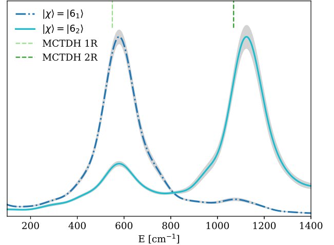
FIG. 6. Semiclassical power spectra in the O-O stretching region, employing harmonic reference states of type (ii), and trajectory sampling as explained in Sec. III E. The straight dashed lines indicate the MCTDH results from Ref. 44. Gray bands behind the curves show the standard deviation of the estimated spectra.
