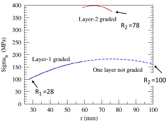
Fig. 13. Improvement in field-generating efficiency of \text{Cos}(\theta) current density distribution using “grading” (left panel). Enhancement of \sigma_{\theta m} associated with grading of a \text{Cos}(\theta) magnet (right panel). Values correspond to those of a \sim 18 T \text{Nb}_3\text{Sn} magnet.
