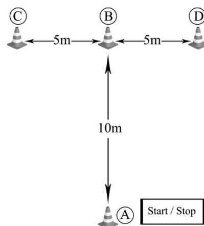
FIG. I. Diagram of T-test.
