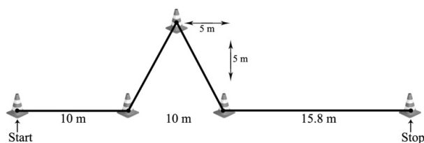
FIG. 2. Diagram of repeated sprint changes of direction.
