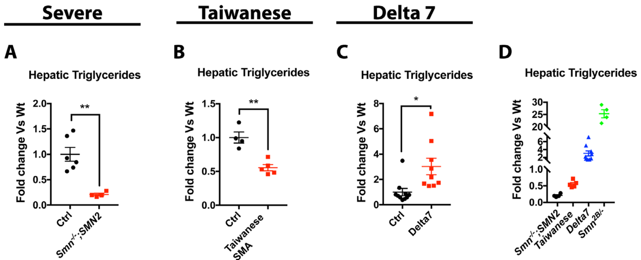
Figure 2. Hepatic triglyceride misregulation is a common feature in different SMA models at symptomatic. Quantification of hepatic triglycerides showed a fivefold reduction in P5 Snm -/- ; SMN2 mice (A), a twofold reduction in P9 Taiwanese mice (B), and a threefold increase in P10 Snm Δ7 mice (C) in comparison to control littermates. Analysis of hepatic triglyceride levels for each SMA mouse model in A–C involved a comparison to their own control ( N value for each experiment is as follows: N = 4–6 for A and B, 9–10 for C, 4–9 for D, unpaired two-sided student's t -test, * P ≤ 0.05 and ** P ≤ 0.01).
