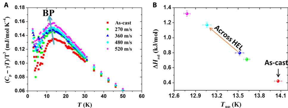
Fig. 5. BPs of the as-cast and rejuvenated metallic glasses. (A) The plot of (C_p - \gamma T)/T^3 versus T in the temperature interval of 2 to 50 K. (B) Correlation between the excess relaxation enthalpy and the BP temperature.
