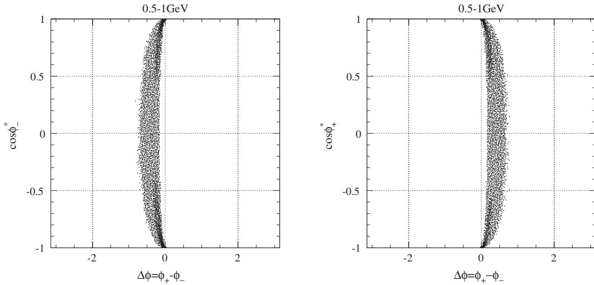
FIG. 13. (Left) Distribution of \cos \phi^* vs \Delta\phi for the N_- sample ( \phi_-^* \in [0, \pi] ) in the (0.5–1.0) GeV/ c^2 mass interval for the \mu^+\mu^-\gamma MC. (Right) The same for the N_+ sample ( \phi_+^* \in [0, \pi] ).
