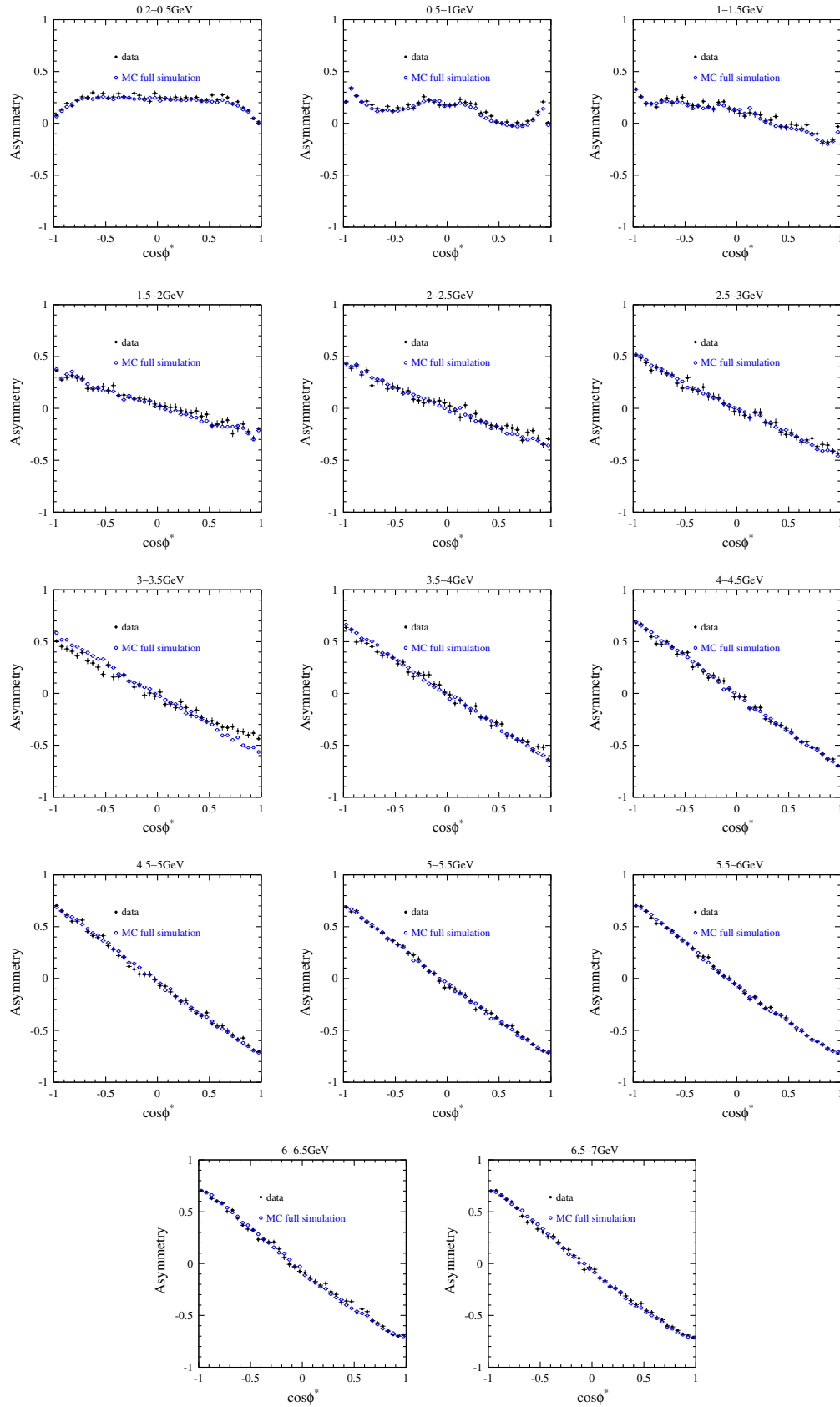
FIG. 14 (color online). Raw charge asymmetry as a function of \cos \phi^* for \mu^+ \mu^- \gamma events in data ( \bullet ) and MC ( \circ ), in various m_{\mu\mu} intervals, after the complete event selection.
