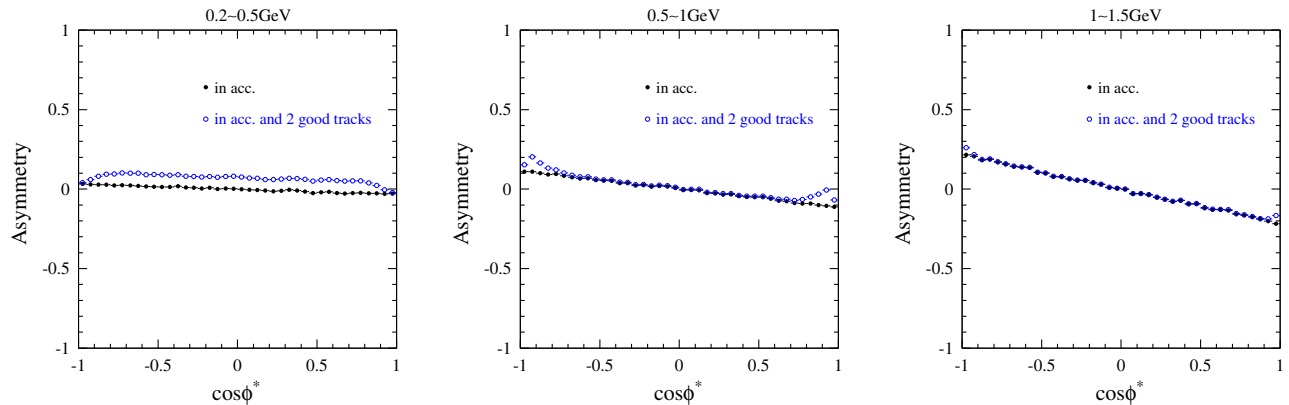
FIG. 10 (color online). Raw charge asymmetry as a function of \cos\phi^* in selected m_{\mu\mu} intervals, for e^+e^- \rightarrow \mu^+\mu^-\gamma MC events with ( \circ ) and without ( \bullet ) reconstruction of two good charged-particle tracks, where the events are already required to be within the kinematic acceptance.
