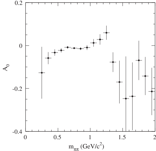
FIG. 22. The fitted slope A_0 of the charge asymmetry for e^+e^- \rightarrow \pi^+\pi^-\gamma at \sqrt{s} = 10.58 GeV, corrected for efficiency within the 20^\circ < \theta_\gamma^* < 160^\circ acceptance in the e^+e^- c.m.
