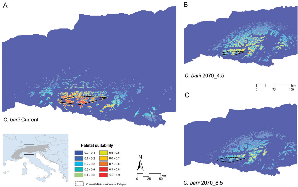
Figure 4. Predicted suitability for Cryptocephalus barii for current and future climatic conditions. Predicted suitability resulting from the Ensemble Modelling process performed over bioclimatic variables for Cryptocephalus barii , with the Minimum Convex Polygon built on the species’ presence sites for A current B 2070 – 4.5 scenario of radiative forcing, and C 2070 – 8.5 scenario of radiative forcing.
