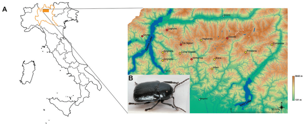
Figure 1. Cryptocephalus barii Burlini, 1948 distribution. A) Geographic location of the Orobic Alps and Cryptocephalus barii distribution. Yellow dots indicate localities where the species was observed, red dots indicate localities investigated with extensive sampling campaigns in which the species was absent (the source map was downloaded from http://www.geoportale.regione.lombardia.it/ and elaborated with QGIS 3.4.1). B) Cryptocephalus barii picture acquired using a Canon 450D camera; the multilayered micrographs were processed with Zerene Stacker (Richland, WA, USA).
