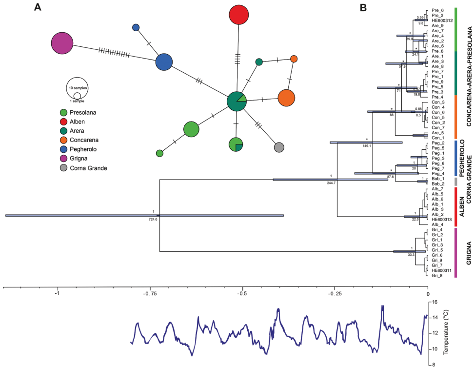
Figure 2. Maximum clade credibility tree and Minimum-spanning haplotype network. A Minimum-spanning haplotype network. Each colour represents a Cryptocephalus barii population. Circles represent the different haplotypes; their diameter is proportional to the haplotypes abundance. B Maximum clade credibility tree. Horizontal blue bars represent 95% HPD age confidence intervals for the nodes. Under the main lineage nodes is reported the divergence time in thousands of years before present. Above the nodes Bayesian posterior probabilities > 0.8 are reported, black asterisks indicate Bayesian posterior probabilities values < 0.80. Vertical coloured bars on the right of the tree indicate monophyletic clades, the colours identify the C. barii populations. Under the tree, in blue, the estimated surface temperature for the last 800,000 years (Hansen et al. 2013).
