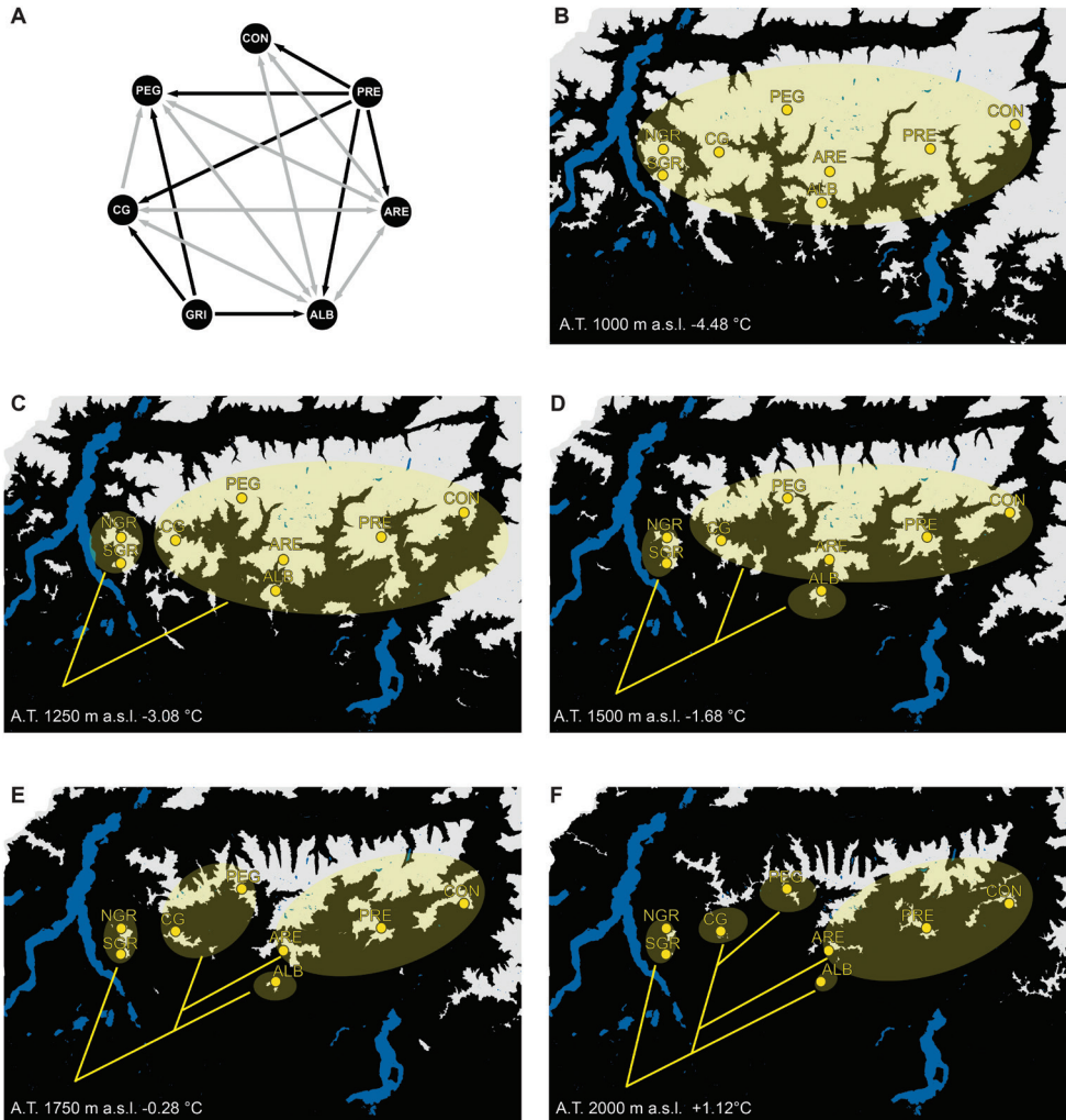
Figure 3. Most likely migration model and altitudinal habitat maps reporting suitable area for the presence of the species during cold periods. A Most likely migration model. Arrows indicate unidirectional flows (in black) and bidirectional flows (in gray) between populations. B–F Suitable altitudinal habitat maps. In light grey are reported the areas suitable for the presence of the species above a certain altitudinal threshold; the yellow ellipses are schematic drawing of Cryptocephalus barii populations; dendrograms showing the divergence events among populations, according to the tree in Fig. 1, are superimposed on the maps. At the bottom left of each map are reported: the minimum elevation at which climatic conditions are suitable for the presence of Cryptocephalus barii (inferred from present knowledge) corresponding to the altitudinal threshold used to draw the suitable areas, and the corresponding estimates of temperature variation in respect to the present. Abbreviations: A.T. = altitudinal threshold; CON = Concarena; PRE = Presolana; ARE = Arera; ALB = Alben; GRI = Grigna; NGR = northern Grigna; SGR = southern Grigna; CG = Corna Grande; PEG = Pegherolo.
