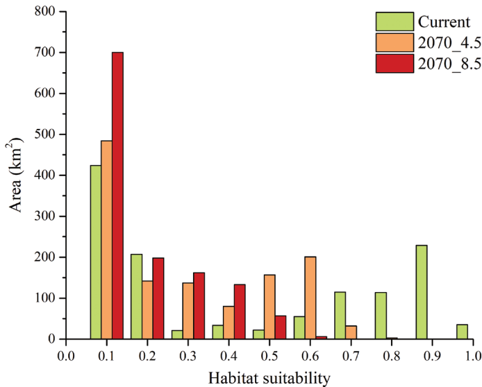
Figure 5. Changes in habitat suitability for Cryptocephalus barii . Histogram reporting classes of habitat suitability calculated within the Minimum Convex Polygon built on Cryptocephalus barii presence sites through Ensemble Modelling process. Areas calculated for current and future climatic conditions (2070, 4.5 and 8.5 scenarios) are reported, respectively, in green, orange and red.
