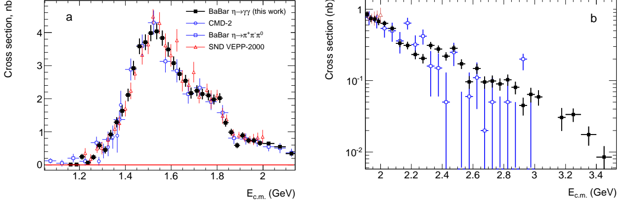
FIG. 11: (color online) The e^+e^- \rightarrow \pi^+\pi^-\eta cross section measured in this work ( BABAR ) in comparison with most precise previous measurements: CMD-2 [9], the independent BABAR (2007) [12], SND [11]) at E_{c.m.} < 2.15 GeV (a) and E_{c.m.} > 1.9 GeV (b).
