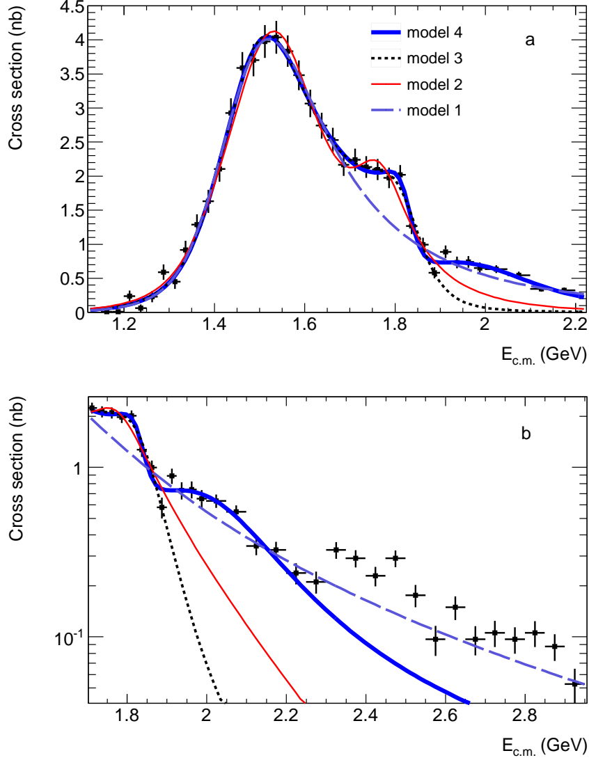
FIG. 12: (color online) The measured e^+e^- \rightarrow \pi^+\pi^-\eta cross section fitted with the four models described in the text.
