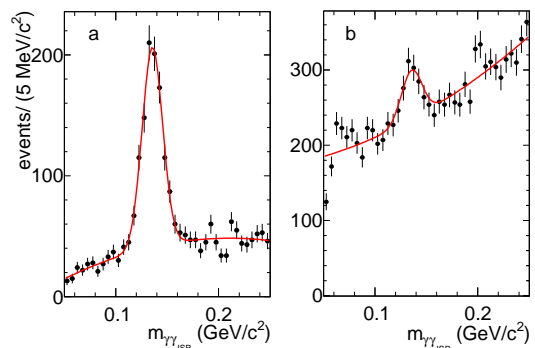
FIG. 4: The distributions of the invariant mass for all combinations of the ISR-photon candidate with any other photon in an event in e^+e^- \rightarrow q\bar{q} simulation (a) and data (b). The curves are the results of the fits described in the text.
