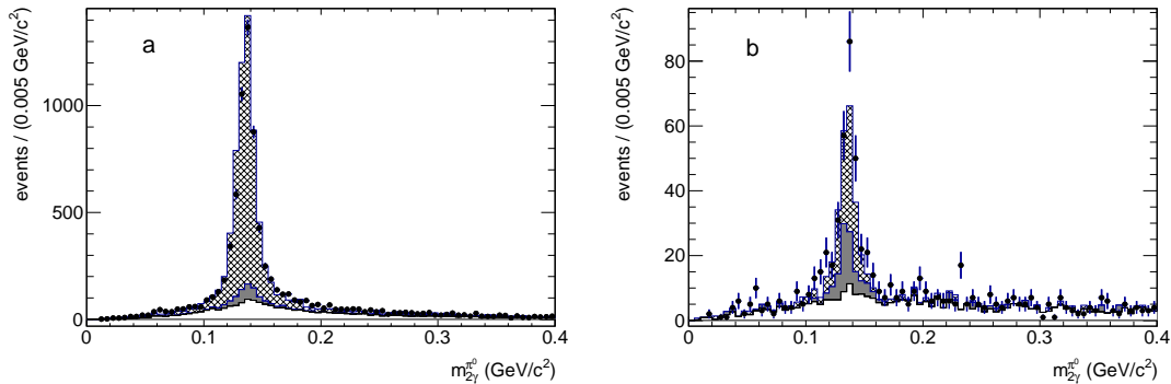
FIG. 3: The distribution of m_{2\gamma}^0 for Region I (a) and for Region II (b). The points with error bars are data. The open histogram represents signal simulation, the shaded and hatched areas shows simulated non-ISR and ISR background contributions, respectively.
