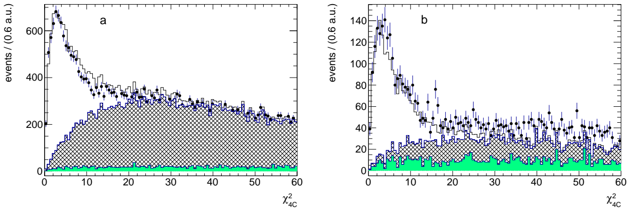
FIG. 2: (color online) The distributions of \chi_{4C}^2 for events from the invariant mass ranges 1.15 < m_{\pi^+\pi^-\eta} < 2.00 \text{GeV}/c^2 (a) and 2.0 < m_{\pi^+\pi^-\eta} < 3.5 \text{GeV}/c^2 (b). The points with error bars are data. The open histogram represents the sum of the simulated distributions for signal and backgrounds events. The shaded histogram represents non-ISR background, while the hatched area shows ISR background.
