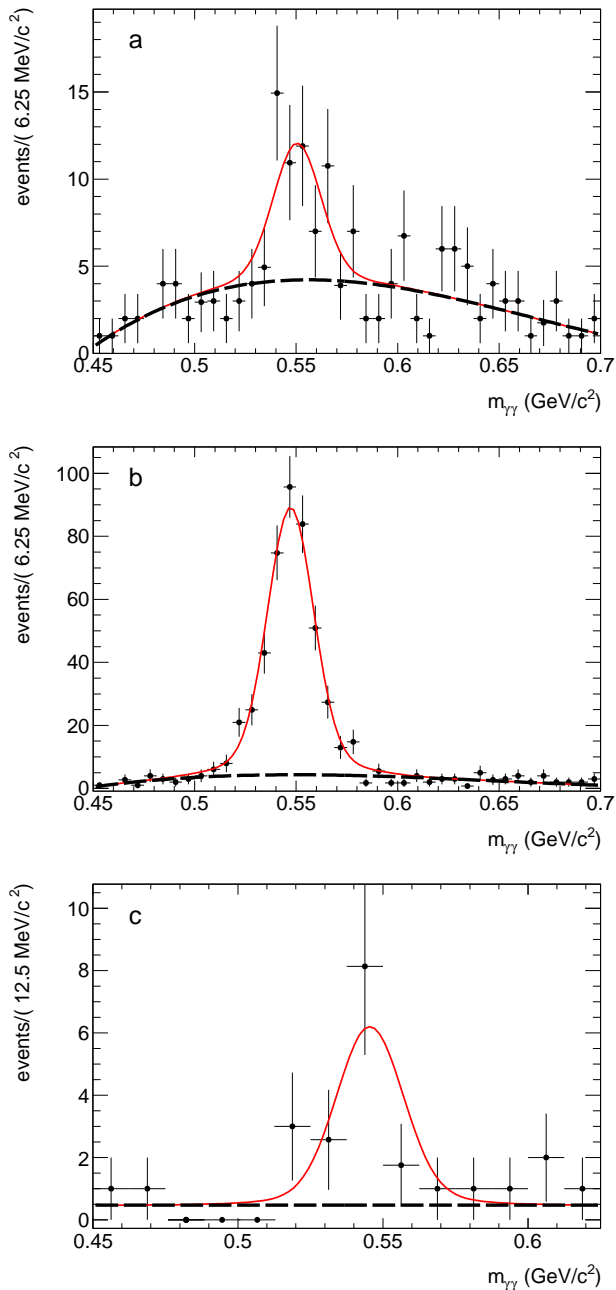
FIG. 6: The two-photon invariant mass spectrum for data events (points with error bars) from the three m_{\pi^+\pi^-\eta} intervals: 1.300–1.325 GeV/ c^2 (a), 1.500–1.525 GeV/ c^2 (b), and 3.4–3.5 GeV/ c^2 (c). The solid curve is the result of the fit described in the text. The dashed curve represents the fitted background.
