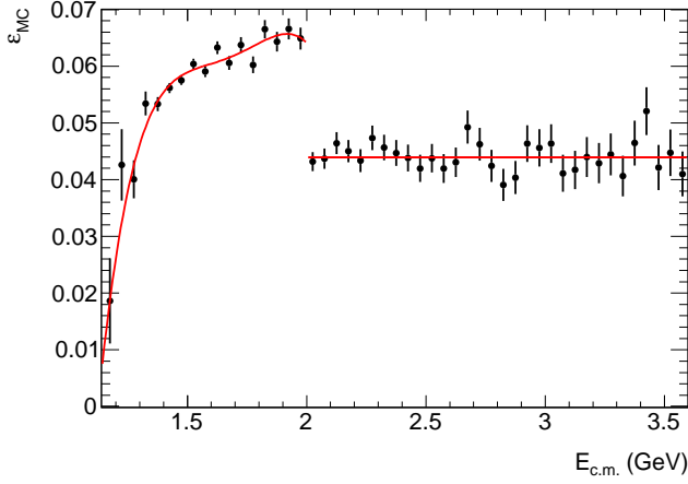
FIG. 10: The detection efficiency \varepsilon_{\text{MC}} obtained using MC simulation as a function of E_{\text{c.m.}} . The lines are fits to a fourth-order polynomial for E_{\text{c.m.}} < 2 GeV and to a constant for E_{\text{c.m.}} > 2 GeV.
