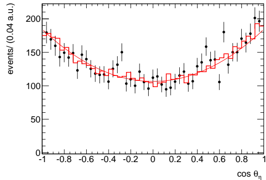
FIG. 9: The \cos\theta_\eta distribution for data (points with error bars) and simulated (histogram) events from the mass range 1.4 < m_{\pi^+\pi^-\eta} < 2.0 \text{ GeV}/c^2 . The curve is the result of the fit described in the text.
