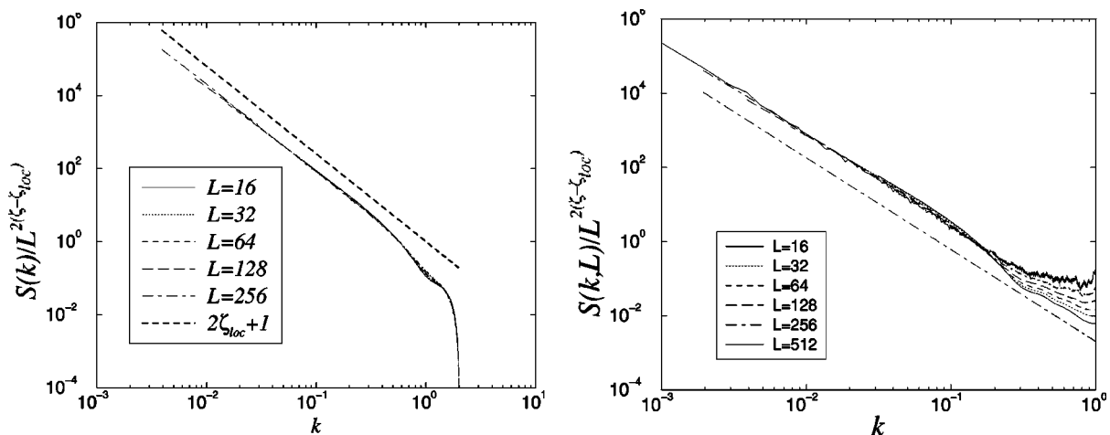
FIG. 4. The power spectrum of the crack S(k, L) for different lattice sizes in log-log scale. The slope defines the local exponent as -(2\zeta_{loc} + 1) . The spectra for all of the different lattice sizes can be collapsed indicating anomalous scaling. Data are shown for diamond (left) and triangular (right) lattices.
