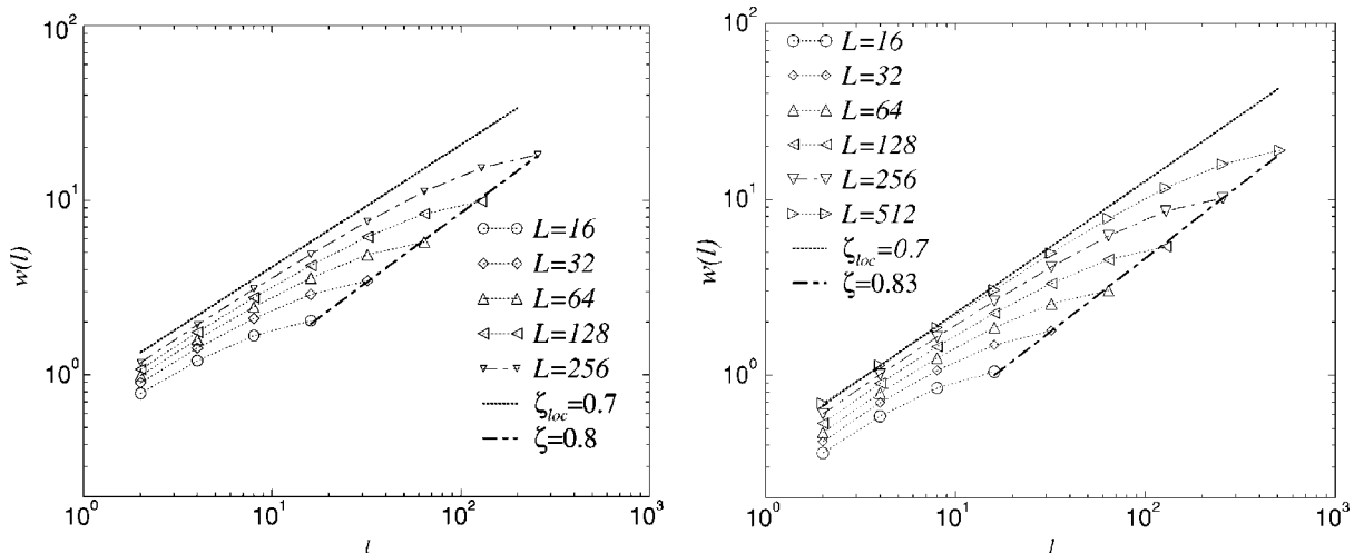
FIG. 2. The local width w(l) of the crack for different lattice sizes in log-log scale. A lines with the local exponent \zeta_{loc} = 0.7 is plotted for reference. The global width displays an exponent \zeta > \zeta_{loc} . Data are shown for diamond (left) and triangular (right) lattices.
