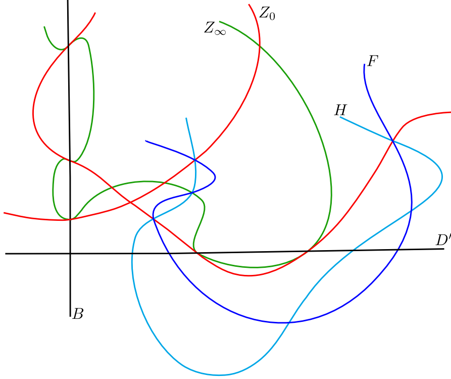
FIGURE 1. The configuration of curves on the generic fiber after Lemma 5.3.5
