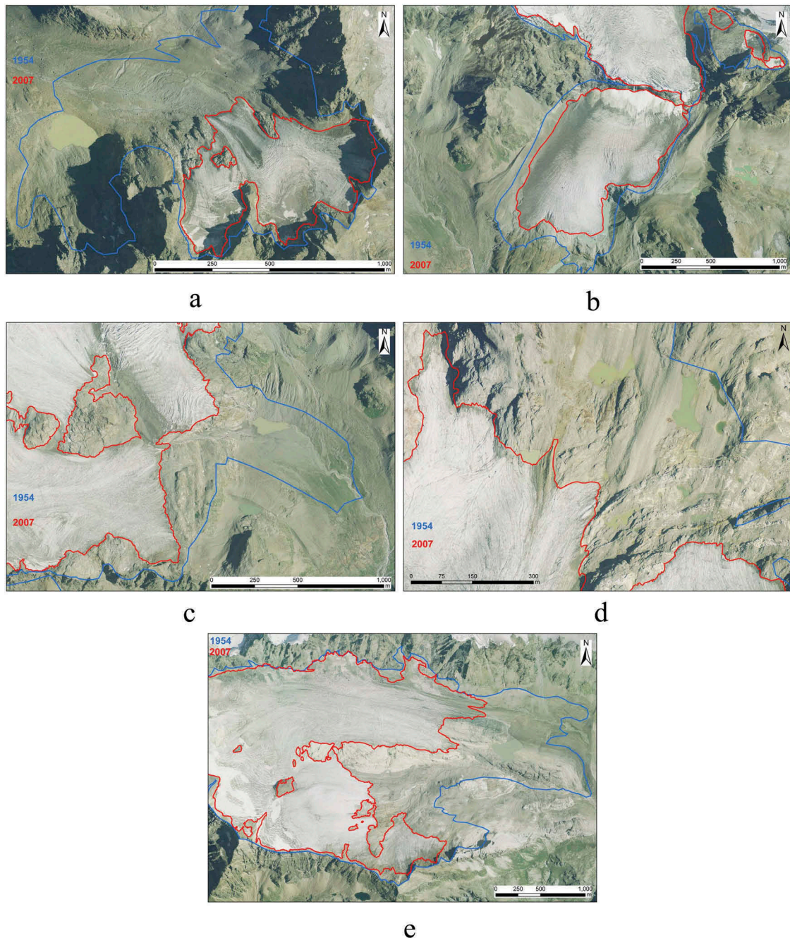
Figure 5. (a) Caspoggio glacier (570,507 E, 5,131,991 N): it is appreciable a newly formed lake in the glacier foreland, moreover unconsolidated sediment and a bare rock area (i.e., roche moutonnée) are also visible in the flat area which is strongly re-worked by meltwater. (b) Fellaria est glacier (573,364 E, 5,135,156 N): a proglacial lake is visible on the left hydrographical side, this was in the past (i.e., 1954) an ice contact lake; moreover also unconsolidated sediment re-worked by meltwater is present. A rock exposure (i.e., roche moutonnée) is also visible. (c) Fellaria Ovest glacier (571,746 E, 5,133,777 N): a newly formed lake is present in the glacier foreland area. Unconsolidated sediment reworked by melting water is also visible together with a wide flat area featuring vegetation (shrubby and grass one) occurrence. (d) Pizzo Scalino glacier (575,946 E, 5,125,974 N): seven newly formed lakes are visible in the glacier foreland area. (e) Scerscen Inferiore glacier (565,177 E, 5,133,396 N): a newly formed lake is present, moreover also unconsolidated sediment and bare rock areas are visible.
