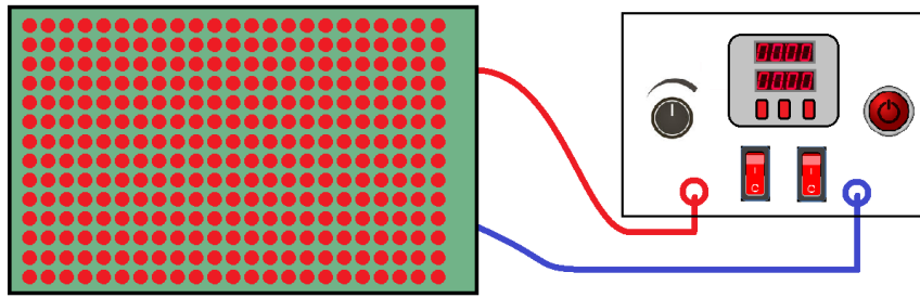
Fig 4.9 Scheme of the LED apparatus. The LED array was connected to a timer to regulate light/dark cycles. With a knob it was possible to regulate the light intensity. On/off button allowed to use continuous light when needed.
