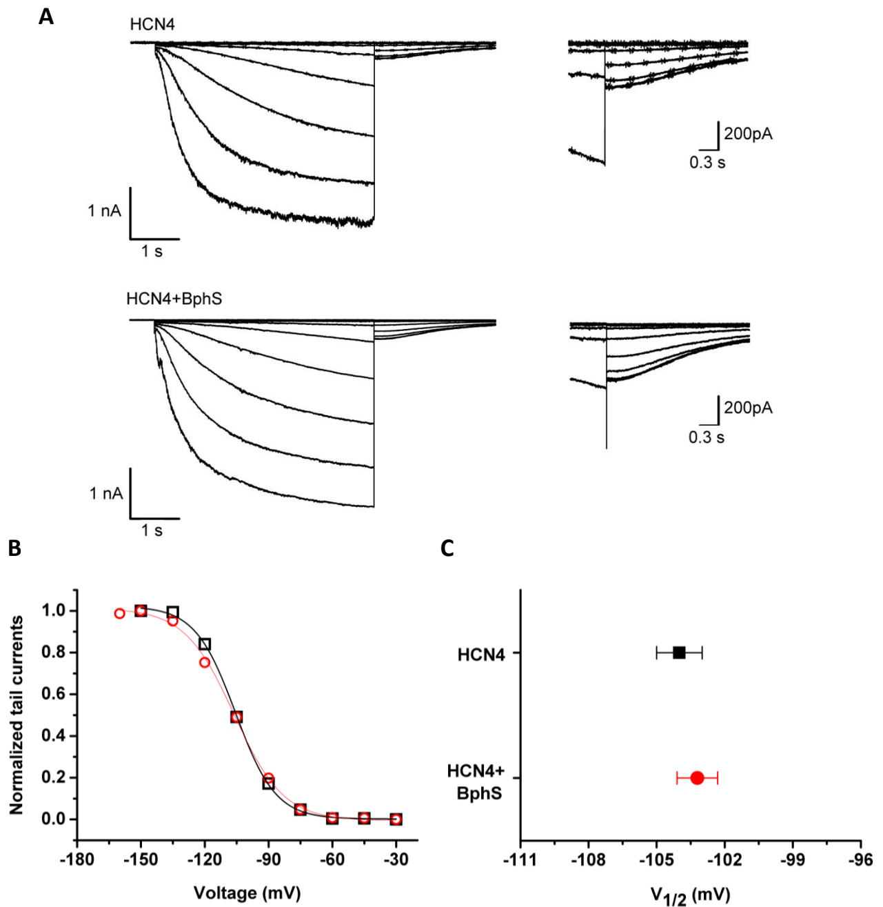
Fig. 4.8 Monitoring the dark activity of BphS. (A) Exemplary current traces obtained by application of voltage protocols in control and BphS-expressing cells. Tail currents (recorded at -40 mV) of each current family are enlarged and reported on the right for each measurement. (B) Normalized tail current amplitudes plotted as a function of the preceding test voltage. Black empty squares: HCN4; Red empty squares: HCN4 + BphS. Data points were fitted with the Boltzmann equation (equation 1). Color code for the fitting is the same used for the data points. (C) Mean \pm S.E. of the V_{1/2} values of HEK293T cells expressing HCN4 or co-expressing HCN4 + BphS. Black squares: HCN4 (N=14); Red squares: HCN4 + BphS (N=12).
