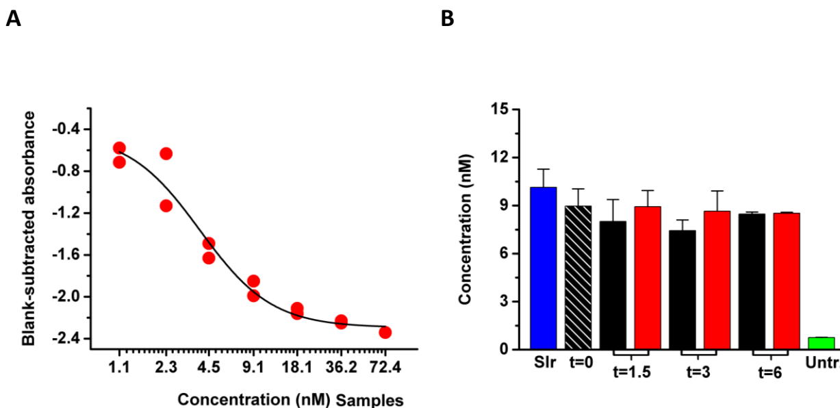
Fig 4.16 Assay of c-di-GMP concentration in HEK293T cells after lysis with Acetonitrile. (A) Blank-subtracted absorbance values of the standards (red dots) measured at 450 nm plotted as a function of their known concentrations (in logarithmic scale). Data points were fitted with a 4PL function (Eq. 2). (B) Concentration values of different cell extracts extrapolated from the calibration curve in (A). Each sample was loaded in three wells of the plate this time: in the graph are reported mean values \pm SE. Samples are identified by the same colors and names used in Fig. 4.15 D.
