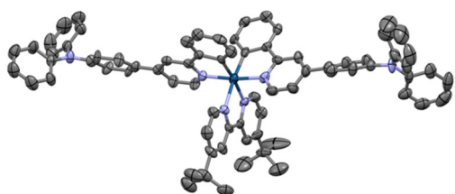
Fig. 1. Solid-state structure of complex 3a . Thermal ellipsoids are drawn at the 50 % probability level. Hydrogen atoms, \text{PF}_6^- counterion and solvent molecules are omitted for clarity.
