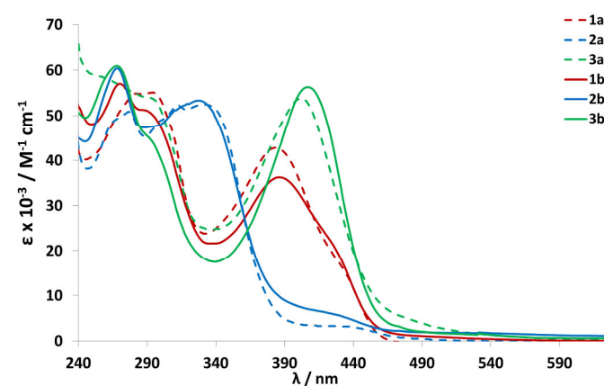
Fig. 2 UV-vis absorption spectra of 1a-3a (in dashed lines) 1b-3b (in solid lines) in \text{CHCl}_3 at 298 K
