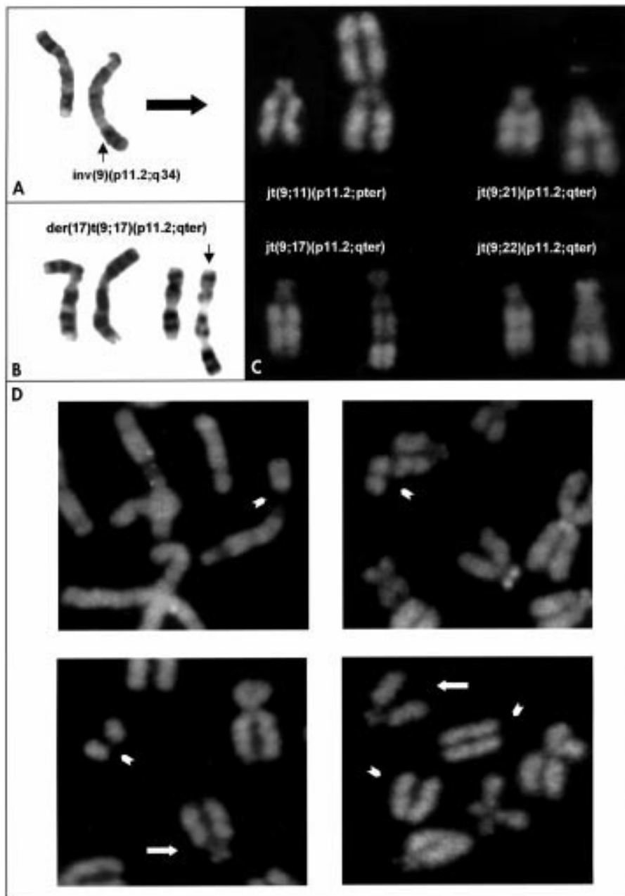
Figure 1 (A) Partial constitutional GTG karyotype from the normal woman showing the inv(9) to the right. (B) GTG banded chromosome 9 and 17 pairs from the woman's child showing the der(17) chromosome leading to 9p trisomy. (C) Partial QFQ chromosome pairs showing a del(9) on the left and, from top to bottom on the right, a few JTs including the one transmitted to the child. (D) Partial QFQ metaphases showing fragility manifestations at inv(9) : the arrows indicate inv(9) with a chromosome gap at 9q34 (top left), inv(9) with a chromatid break at 9q34 (top right), del(9p) (bottom left) and the ace in the same metaphase, del(9p) and two ace i(9)(p10) (confirmed by FISH using specific 9p telomeric probes) (bottom right).
