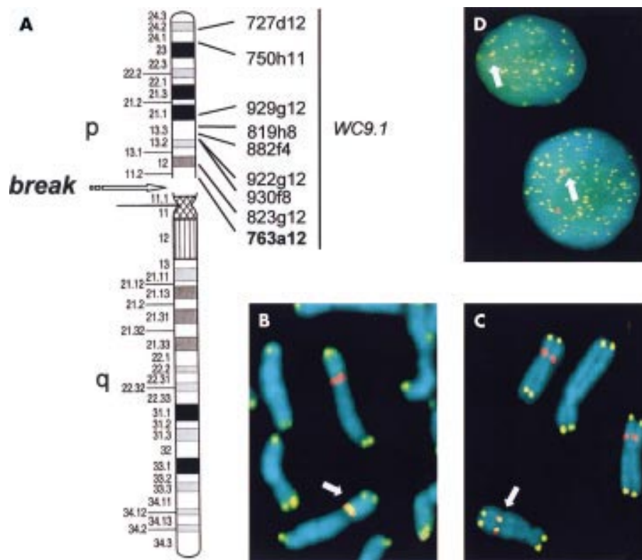
Figure 3 (A) Ideogram of chromosome 9: the arrow indicates the p breakpoint underlying the formation of inv(9) . The YAC clones from the WC9.1 contig used in the FISH experiments are indicated; YAC y763a12 (which is close to the p breakpoint) is in bold. Dual FISH of y763a12 and all of the human telomere probes show two overlapping interstitial signals on mother inv(9) (B) and child der(17) (C). Merging of the two signals is also observed on the mother's interphase cells (D), thus showing the close contiguity of the target sequences.
