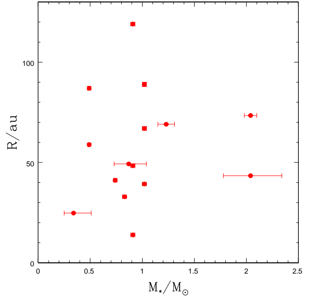
Figure 4. Scatter plot showing the gap location R (y-axis) vs. the central star mass M_* (x-axis) for the putative planets in Long et al. (2018).
