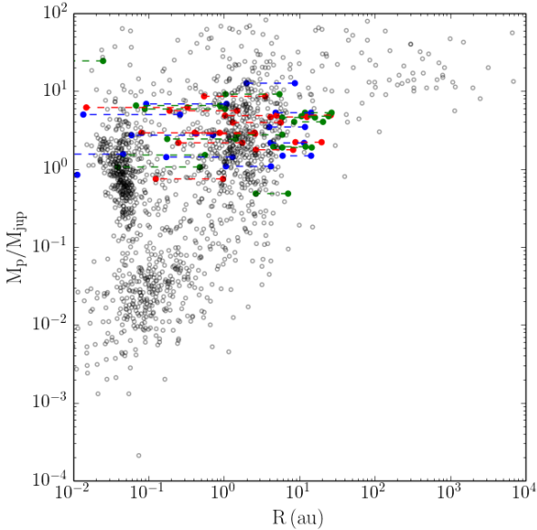
Figure 5. Same as Fig. 1 but where the points indicate the expected final mass and location of the putative planets inferred in Long et al. (2018) (red), Zhang et al. (2018) (green) and Bae et al. (2018) (blue) after 3 and 5 Myr of planet evolution. The dashed lines indicate the range of planet locations after a total time in the range [3,5] Myrs. Planetary accretion and migration lead to a redistribution of planet properties that mostly populates the branch of cold Jupiters.
