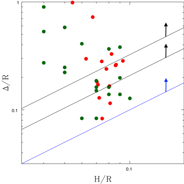
Figure 2. Measured gap widths vs. disc aspect ratio (as estimated from Eq. (5)) in the Long et al. (2018) (red points) and in the Zhang et al. (2018) (green points) samples. The two black lines indicate the range [2.1 - 3.2]H/R above which the gap width is expected to lie if the dust is strongly coupled to the gas ( St \ll 1 ). The blue line indicates the relation \Delta = H , that is the minimum gap width expected for dust with St \sim 1 .
