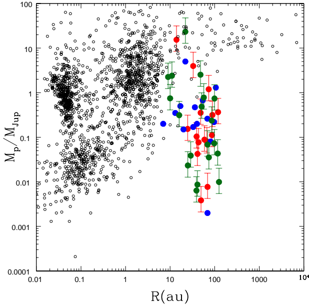
Figure 1. Plot of mass (y-axis) M_p vs. separation from the central star R (x-axis) of the (empty circles) currently known exoplanets (retrieved from the exoplanet.org database) compared to those obtained from the sample in Long et al. (2018) (red points) and Zhang et al. (2018) (green points) using Eq. (2), and those collected by Bae et al. (2018) (blue points). Error bars in the planet masses indicate the uncertainty in the proportionality factor between gap width and planet’s Hills radius, assumed to be in the range [4.5 – 7].
