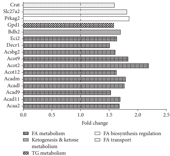
FIGURE 3: Lipid metabolism-related transcriptome in obese and lean hearts. Gene expression profile was evaluated using the rat Fatty Acid Metabolism RT 2 Profiler PCR Array. Genes that showed a fold change > 1.5 in obese vs. lean groups are represented and grouped according to their biological function.
