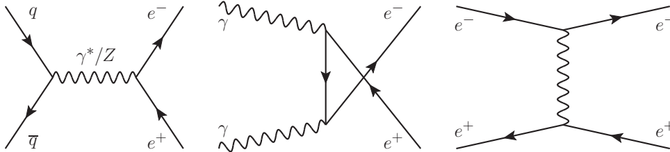
Figure 11. Representative diagrams for partonic processes in e^+e^- production.
