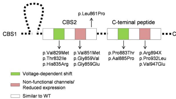
FIGURE 6 Clustering of MC mutations. Schematic drawing showing clusters of CIC-1 mutations within CBS2 and C-terminal peptide subdomains that share the same functional defect
