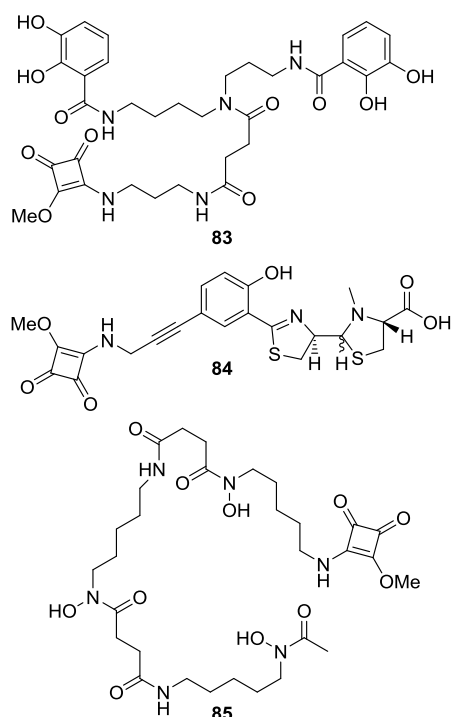
Figure 26. Siderophore-monomethylsquarate esters 83–85 . [161]
