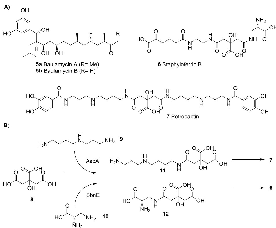
Figure 4. A) Baulamycin A 5a , a natural product discovered in screens for staphyloferrin and petrobactin-family siderophore inhibitors. B) Baulamycins inhibit the AsbA -catalyzed condensations of citrate 8 with spermidine 9 in petrobactin 7 biosynthesis, and the analogous SbnE -catalyzed condensation of 8 and diaminopropionic acid 10 in staphyloferrin 6 biosynthesis.
