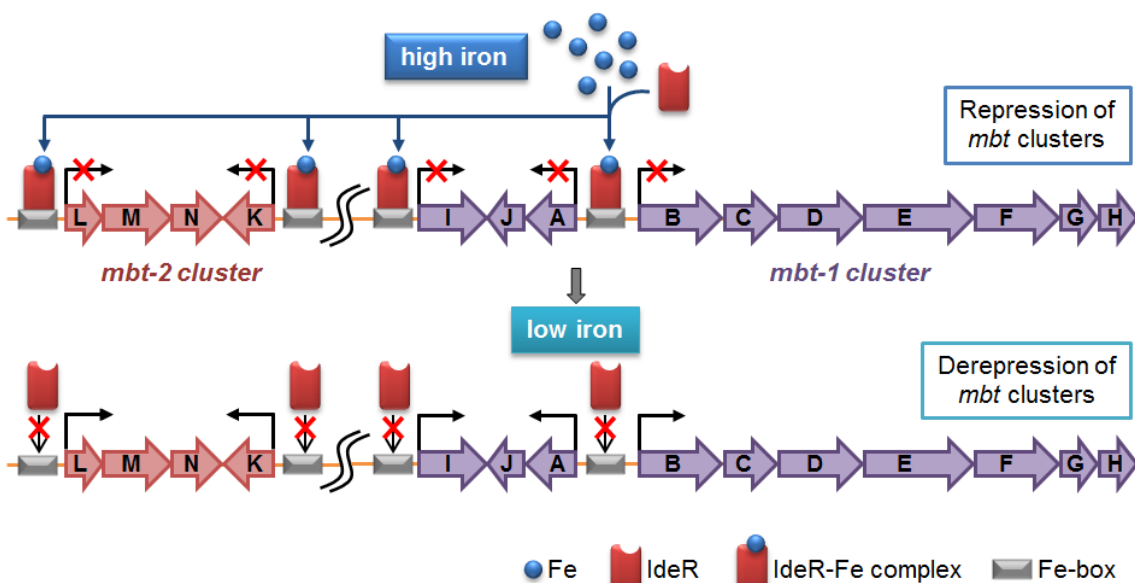
Figure 2. Control of gene expression via IdeR by \text{Fe}^{2+} concentration. In the presence of high iron concentrations
