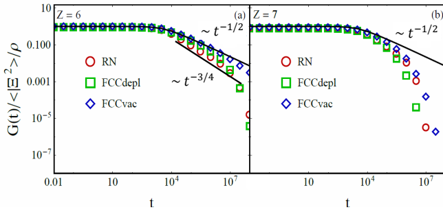
FIG. 4. G(t) of our three model systems for Z = 6 (left) and Z = 7 (right). We have indicated the different scaling ranges. One can see that the power-law scaling, which is present on 3 – 4 orders of magnitude in time for Z = 6 , breaks down for Z = 7 . This is due to the expanding Debye \sim \omega^2 regime in the DOS, see text.
