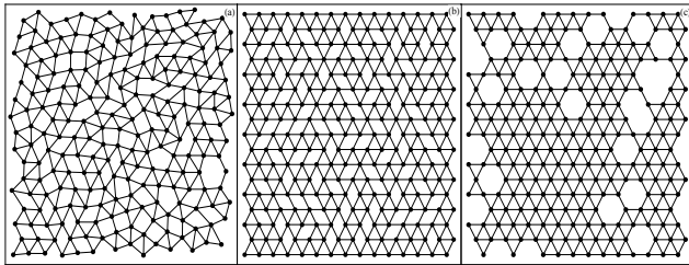
FIG. 1. Two dimensional schematic of our 3D model systems. (a) the random network, (b) the fcc lattice with randomly cut bonds and (c) the fcc lattice with randomly removed atoms.
