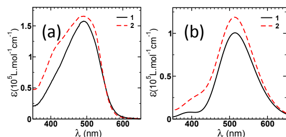
Fig. 1. UV-vis absorption spectra of compounds 1 and 2 in DCM (a) experimental spectra and (b) calculated spectra for a HWHM=2000 \text{cm}^{-1} .
