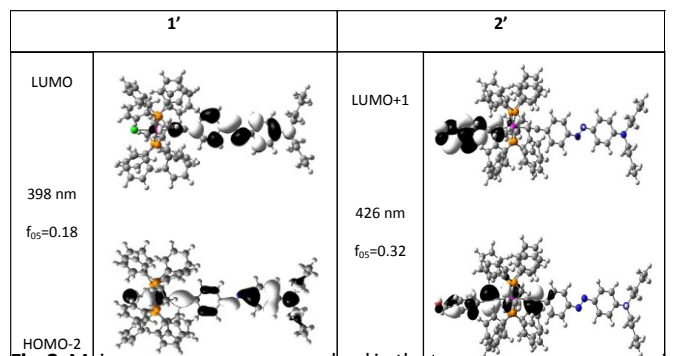
Fig. 2. Main molecular orbitals involved in the two lowest lying electronic transitions having sizeable oscillator strength ( f_{0i} ) for compounds 1' and 2' (models of 1 and 2 , see Computational Details). Corresponding wavelengths are also given. Both geometries and properties have been computed in the presence of solvent (DCM). The weight on the Ru atom amounts to 17 and 19% respectively in the HOMO and HOMO-2 of compound 1' and to 15 and 38% in the HOMO and HOMO-1 of compound 2' .
