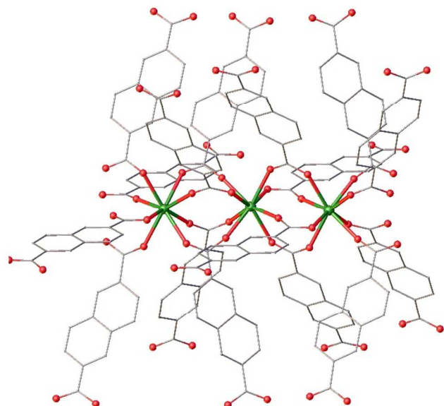
Figure 1. Rows of connected thorium atoms along the [101] direction in \text{Th}(\text{NDC})_2 MOF. Hydrogens are omitted for clarity. Th (green), O (red), C (grey).
