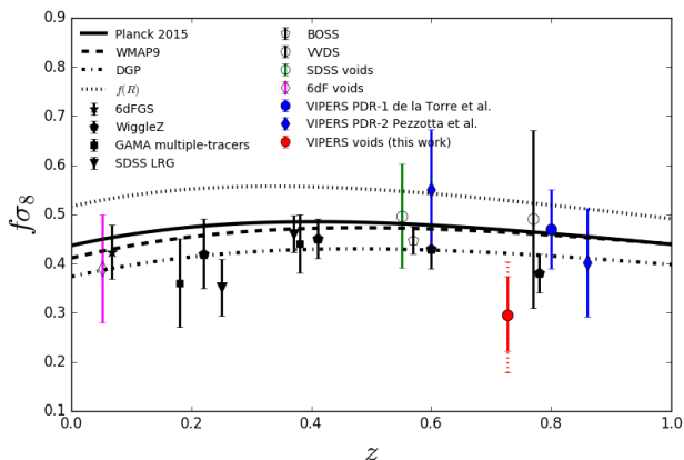
Fig. 12: Comparison to other estimates of the growth rate (Beutler et al. 2012; Blake et al. 2011, 2013; Samushia et al. 2012, 2014; Guzzo et al. 2008). Of particular interest are the measurement using conventional galaxy clustering techniques on VIPERS PDR-1 (blue filled circle: de la Torre et al. 2013); the measurement using voids in SDSS (green open circle: Hamaus et al. 2016); and the measurement using voids in 6dF (magenta diamond: Achitouv & Blake 2016).
