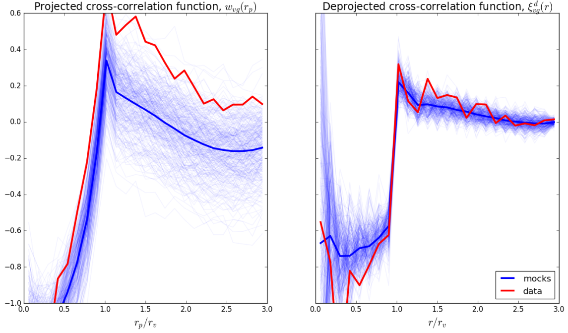
Fig. 6: Projected (left hand panel) and deprojected (right hand panel) void-galaxy cross-correlation functions for mock catalogues (blue) and the VIPERS data (red). Here the minimum void radius used is 8 h^{-1}\text{Mpc} . The mock catalogues were not constructed with a mind to accurately reproducing void properties, therefore the fact that there are some inconsistencies between mock and data void profiles is to be expected.
