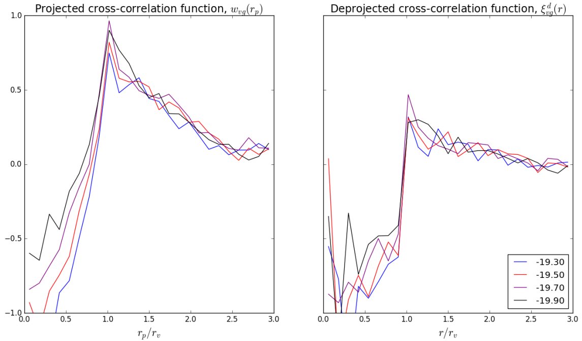
Fig. 10: Projected cross-correlation functions (left hand panel) and deprojected density profiles (right hand panel) for voids in VIPERS, found in volume limited catalogues with different magnitude cuts. When a brighter magnitude cut is used to define the volume limited catalogue the voids found are less empty and thus the interior void profile changes.
