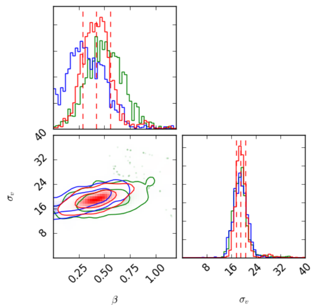
Fig. 11: MCMC contours for two parameter RSD model fit to VIPERS. The green contours indicate the fit to W4, the blue to W1, and the red contours are from the combination of the two fields. There is no significant tension between the two fields.
