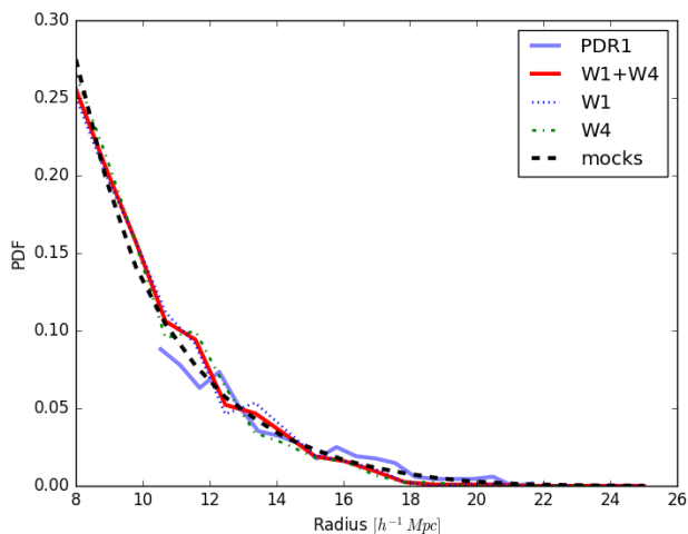
Fig. 2: The normalised histogram of void radii in this data set (red solid line) compared to those in the mock catalogues (black dashed line). The blue and green dotted lines show the two individual fields in this data set. The distribution of void sizes in the data is in very good agreement with the mocks. The histogram of void sizes in Micheletti et al. (2014) is also plotted (blue solid line). Note that this has been renormalised to account for the change in minimum void radius in this work.
