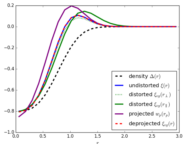
Fig. 3: Model for the void-galaxy cross-correlation function. The integrated density contrast, Equation (5), is plotted as a black dashed line. The one dimensional void-galaxy cross-correlation function, without redshift space distortions, is plotted as a solid blue line. The void-galaxy cross-correlation function with redshift space distortions, as seen directly along the line of sight, is plotted as a solid green line. The dotted green line is the same model as seen tangential to the line of sight. The projected cross-correlation function is plotted as a purple line. The deprojection is plotted as a red dashed line, it matches the blue line very closely. The values of the model parameters are \beta = 0.8 , \sigma_v = 13.4 \text{ km s}^{-1} (h^{-1} \text{Mpc})^{-1} , \delta_c = -0.8 , r_v = 0.9 , \alpha = 3.0 .
