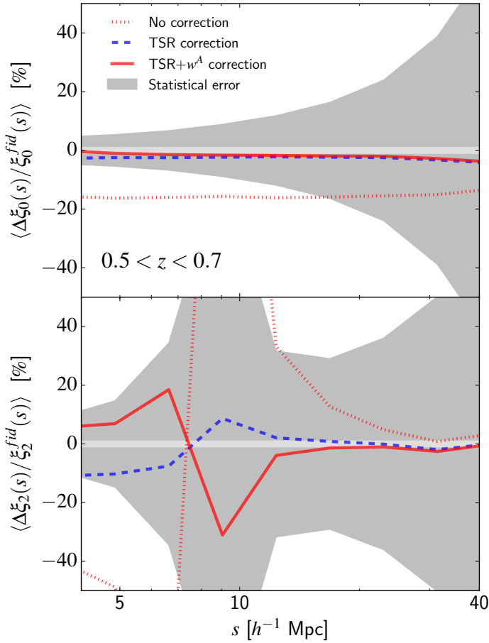
Fig. 4. Relative systematic errors on the correlation function monopole (top panel) and quadrupole (bottom panel) at 0.5 < z < 0.7 and effects of target sampling rate (TSR) and angular pair weighting ( w^A ) corrections. The grey shaded areas represent the relative statistical error expected in the survey, while light grey band mark \pm 1\% relative uncertainties for reference.
