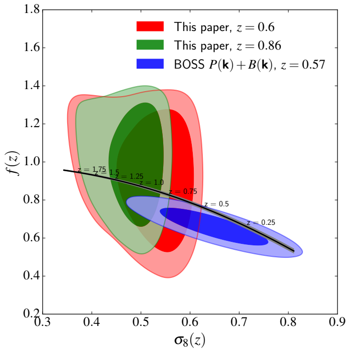
Fig. 16. Joint (f, \sigma_8) constraints at different redshifts. The combined RSD and galaxy-galaxy lensing posterior likelihood contours at 1\sigma and 2\sigma and those from Gil-Marín et al. (2017), obtained by combining redshift-space power spectrum and bispectrum information in the BOSS survey, are presented. The solid curve and associated grey shaded area correspond to the expectations and 68% uncertainty for General Relativity in a \Lambda CDM background model set to TT+lowP+lensing Planck 2015 predictions (Planck Collaboration et al. 2016), as a function of redshift from z = 2 to z = 0 .
