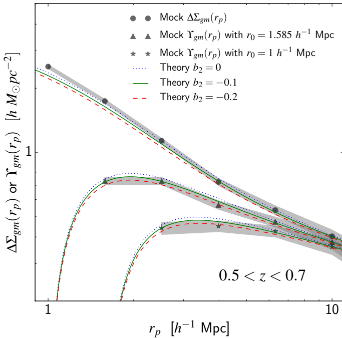
Fig. 7. Comparison of differential excess surface density \Delta\Sigma_{gm} and annular differential excess surface density \Upsilon_{gm} predictions in the mocks (points and shaded regions) and by our theoretical model (curves) at 0.5 < z < 0.7 . The mock predictions correspond to the mean signal among the mock realizations (points) and its associated 1\sigma error (shaded region). The curves show the theoretical predictions for the fiducial parameters of the mocks, varying only the b_2 parameter as labeled.
