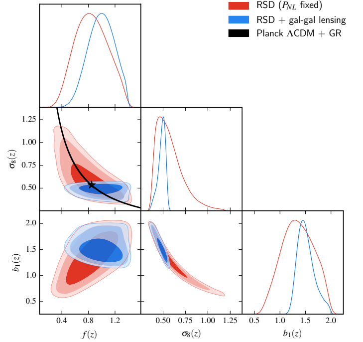
Fig. 15. Same as Fig. 14 but for the redshift interval 0.7 < z < 1.2 .
