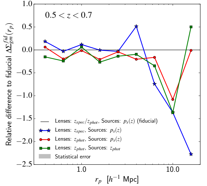
Fig. 2. Relative difference between various estimates of \Delta\Sigma_{gm} , based on different assumptions for source and lens redshifts, and the fiducial estimate in the data at 0.5 < z < 0.7 . The quantity shown in the figure is \Delta\Sigma_{gm}/\Delta\Sigma_{gm}^{\text{fid}} - 1 as a function of the projected separation r_p . The fiducial estimate \Delta\Sigma_{gm}^{\text{fid}} is that obtained by using Eq. 13, which includes the individual redshift probability distribution function p_s(z) of the sources, and for the lenses, the VIPERS spectroscopic redshift ( z_{\text{spec}} ) when available or the CFHTLenS maximum likelihood photometric redshift ( z_{\text{phot}} ) otherwise (see text). It corresponds to the adopted estimate for the analysis. The grey shaded area represents the relative statistical error expected in the survey.
