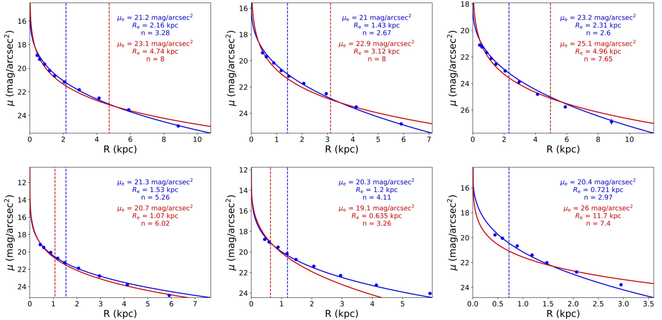
Figure 5. Sérsic profiles of the 6 galaxies showing the highest scatter with respect to the best-fitting linear relations in Fig. 4 are shown. Blue solid lines are the Sérsic profiles built with the best-fitting parameters we estimate in Sect. 3.3. Red solid lines are the Sérsic profiles built with the GALAPAGOS run best-fitting parameters. Blue points are aperture magnitudes in the F814W waveband. Colour-coded dashed lines mark the estimated effective radii. On the top right of each plot, the best-fitting parameters colour-coded by the method are shown.
