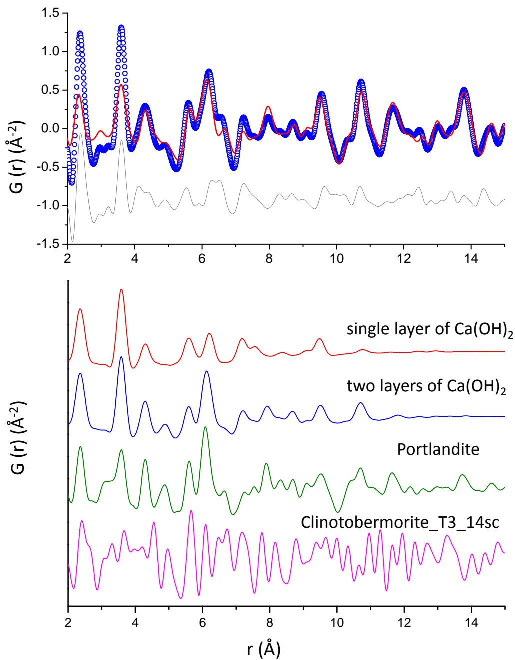
Supplementary Figure 8. Experimental (blue circles) and fitted (red solid line) PDF patterns for \text{C}_3\text{S}_{3\mu\text{m}_080\_arrested:16d} in the 2 to 15 \text{\AA} r -range with three components: crystalline portlandite, unreacted alite and clinotobermorite. Difference curve is shown as a grey line which clearly shows the presence of an amorphous constituent. Simulated PDF curves for a monolayer (red) and a double layer (blue) calcium hydroxide, crystalline portlandite (green) and clinotobermorite T3_14sc (pink) are also included.
