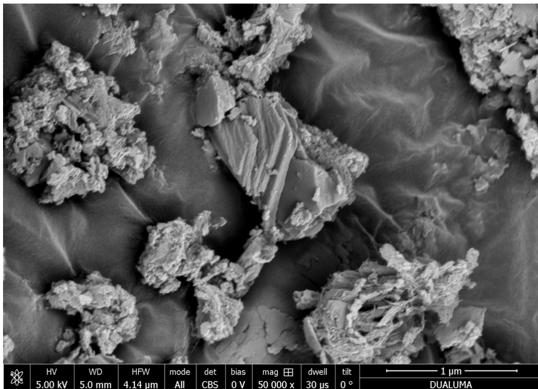
Supplementary Figure 6. Field emission gun scanning electron (FEGSEM) micrograph for C 3 S_3μm_080_arrested:16d.
