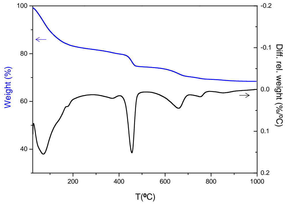
Supplementary Figure 9. Thermogravimetric data for C 3 S 3µm_080_arrested:16d .
