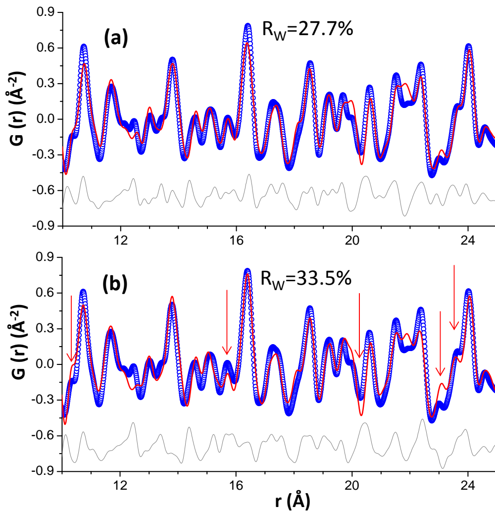
Supplementary Figure 7. Experimental (blue circles), fitted (red lines) and difference (grey lines) PDF patterns for C3S_3 \mu\text{m} _080_arrested:16d from 10 to 25 \text{\AA} using (a) clinotobermorite T3_14sc and (b) Jennite. The arrows highlight interatomic distance features poorly fitted by the Jennite structural description.
