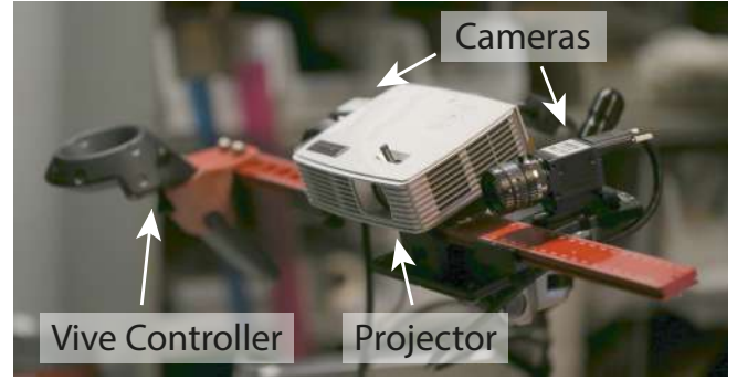
Fig. 11. Hardware setup
