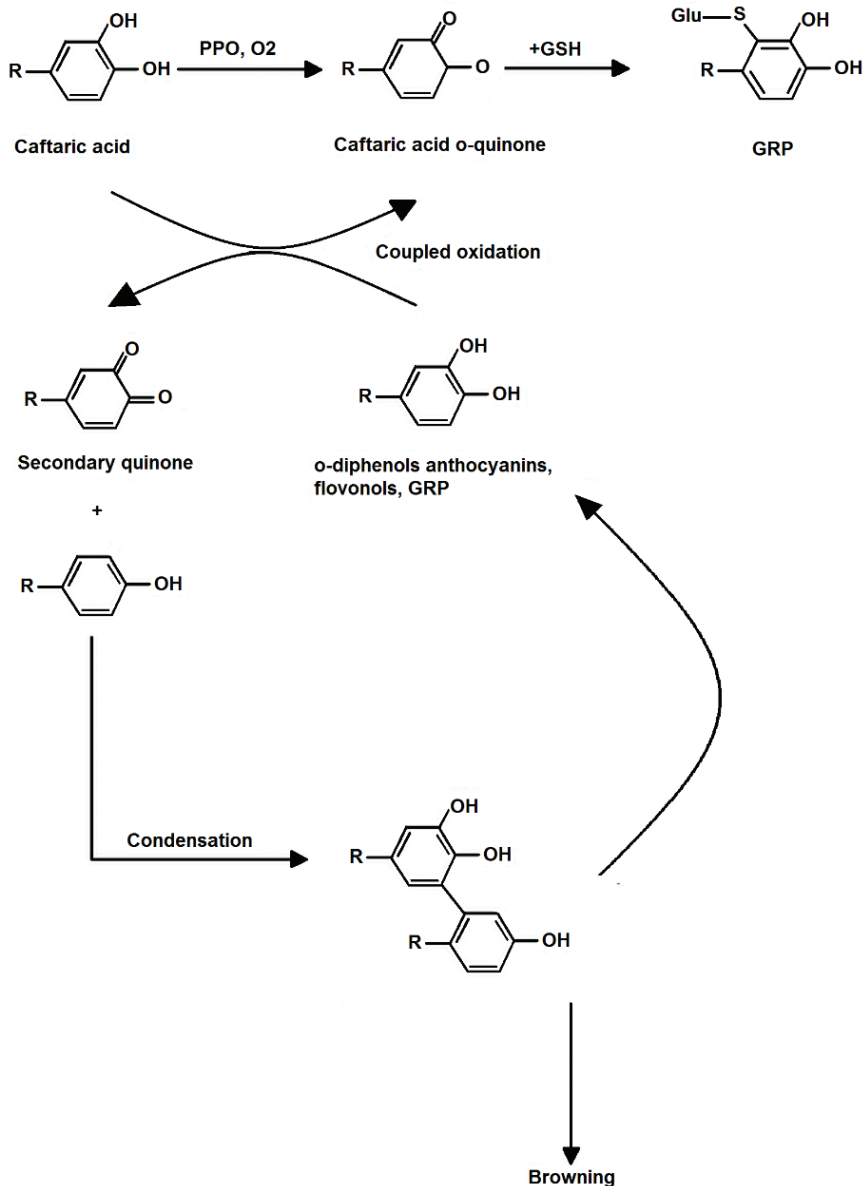
Figure 2. Scheme of GRP and browning compound formation [100–102].
