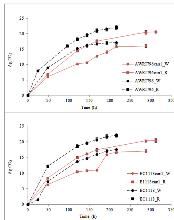
FIGURE 5 | Production of CO 2 by S. cerevisiae wild type (AWRI796 and EC1118) and recombinant strains (AWRI796 can1 and EC1118 can1 ) in oenological conditions. R, Cabernet Sauvignon must; W, Chardonnay must. Data are expressed by means of three replicates and standard deviation (±SD).
