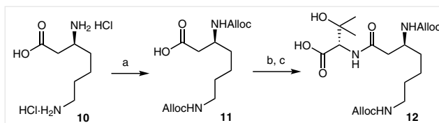
Scheme 2 Synthesis of dipeptide 12 . Reagents and conditions: (a) allyl chloroformate, K_2CO_3 , H_2O , 0^\circ C to r.t., 16 h, 73%; (b) NHS, EDC-HCl, DMF, r.t., 16 h; (c) 3-hydroxy-L-valine, Et_3N , dioxane- H_2O (2:1), r.t., 2 h, 86% (over 2 steps).
