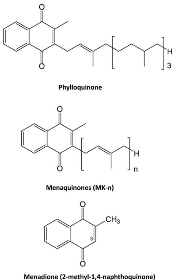
Figure 1: Structures of phylloquinone (vitamin K1) and menaquinones (MKs or vitamin K2). Menadiene (vitamin K 3 ) represents the basic structure common to K1 and K2. Menadiene is available as a synthetic form of vitamin K.
