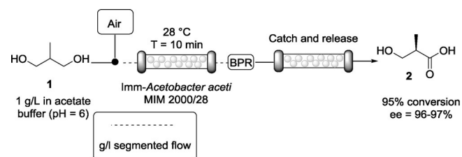
Scheme 2. Biocatalyzed heterogeneous oxidation of prochiral 2-methyl-1,3-propanediol ( 1 ) and in-line purification of the product through a catch-and-release protocol.
