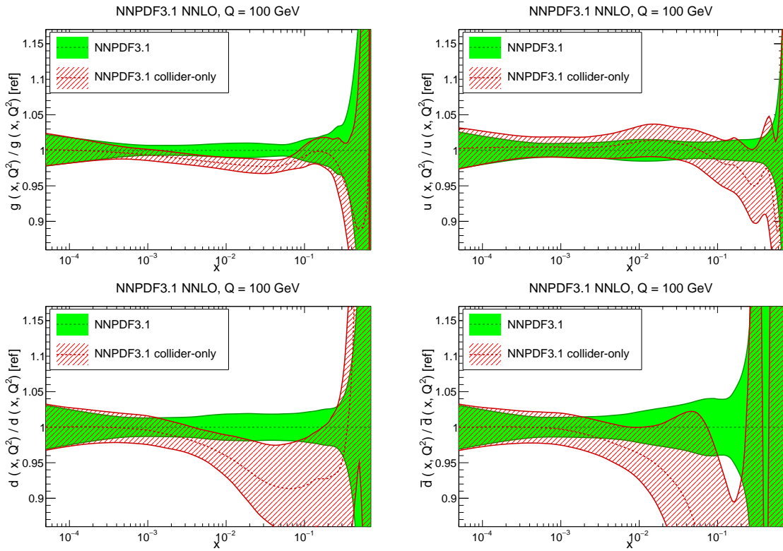
Figure 4.34: Same as Fig. 4.4 but now only keeping collider data. Results are shown for the gluon (top left), up (top right), down (bottom left) and antiquark (bottom right).
