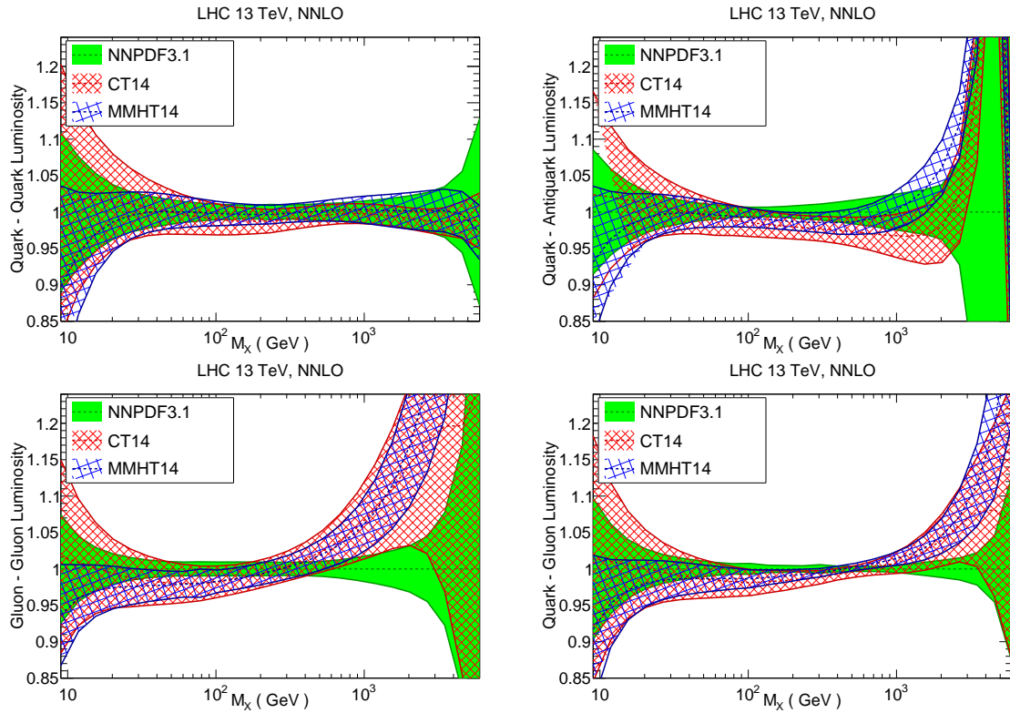
Figure 5.10: Same as Fig. 5.8, now comparing NNPDF3.1 NNLO to CT14 and MMHT14.
