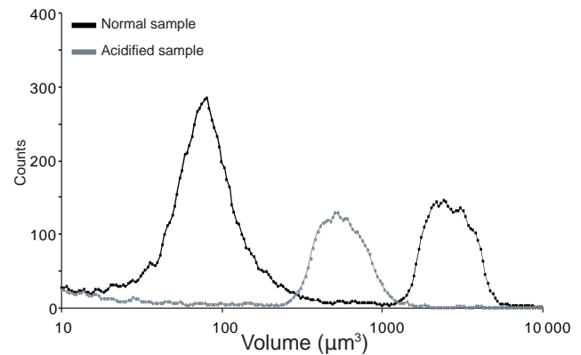
Figure 1. Example of Multisizer volume spectra. Black line: spectra of C. pelagicus population (coccolith spectrum and coccosphere spectrum); gray line: C. pelagicus coccolith-free cell after treatment with HCl.
